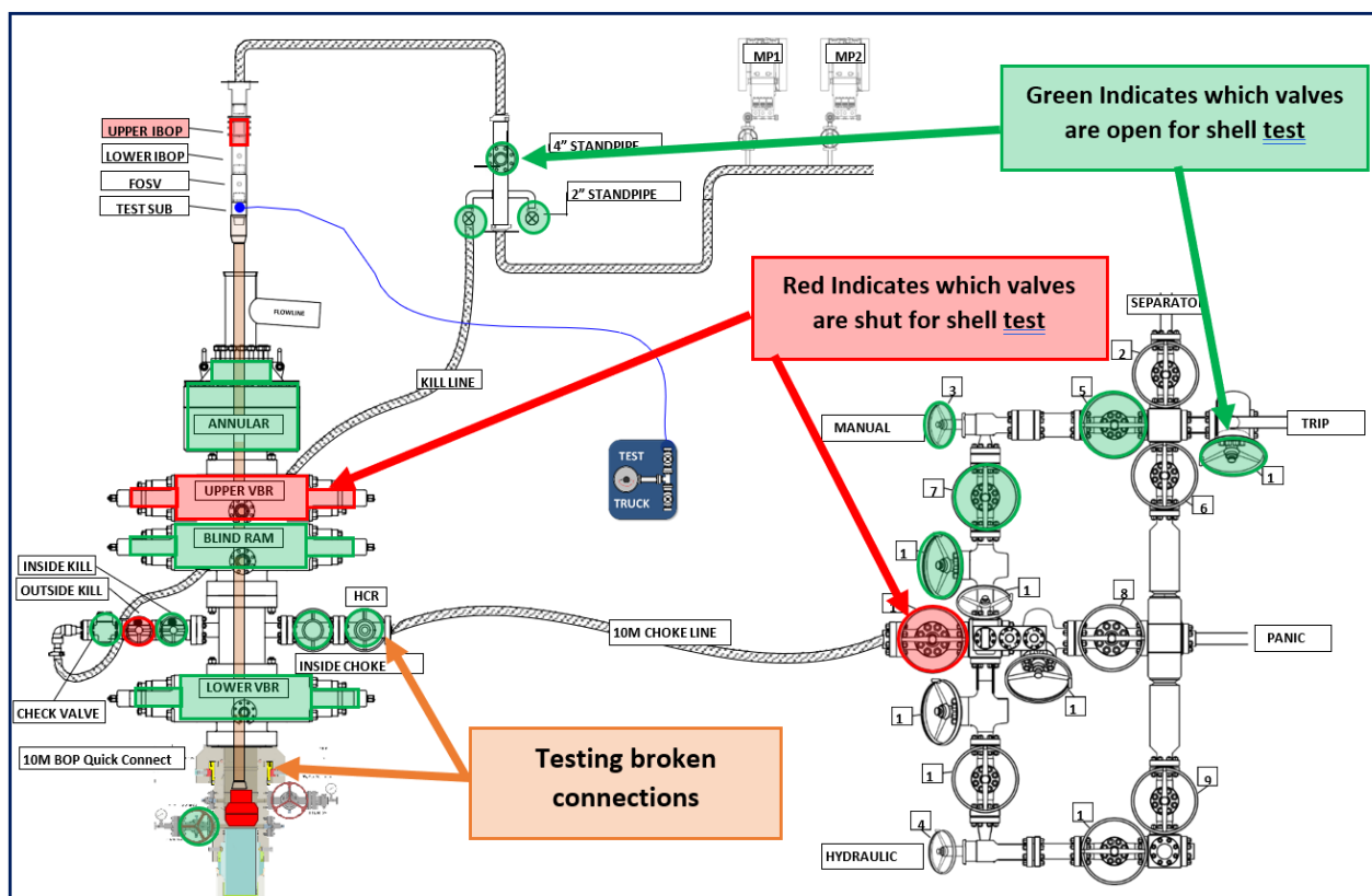
Figure 4: Shows which valves are shut/open for the shell test, testing both broken connections
