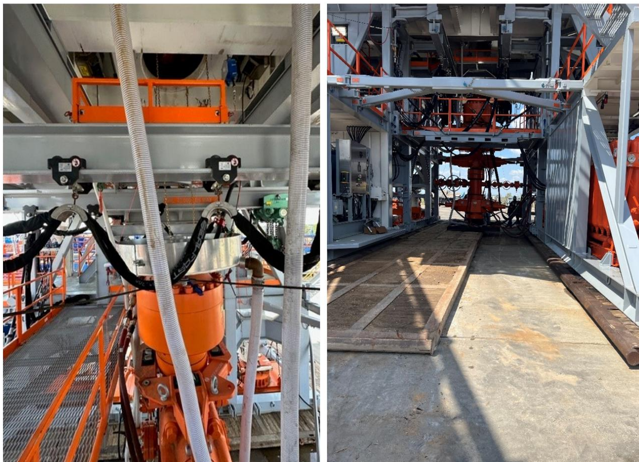
Figures 1 & 2: BOP winch system picture with walking capabilities.
