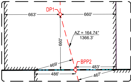
DETAIL VIEW SCALE: 1" = 600'
