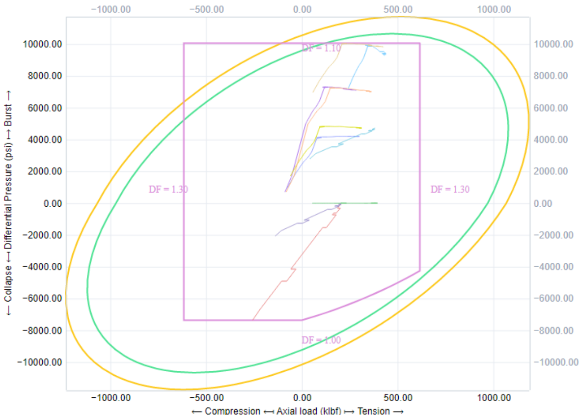
CASING TRIAXIAL: 7-5/8-inch, 29.7 lb/ft, P110-ICY, BTC, MCBU (28 - 11578.58 ft)
