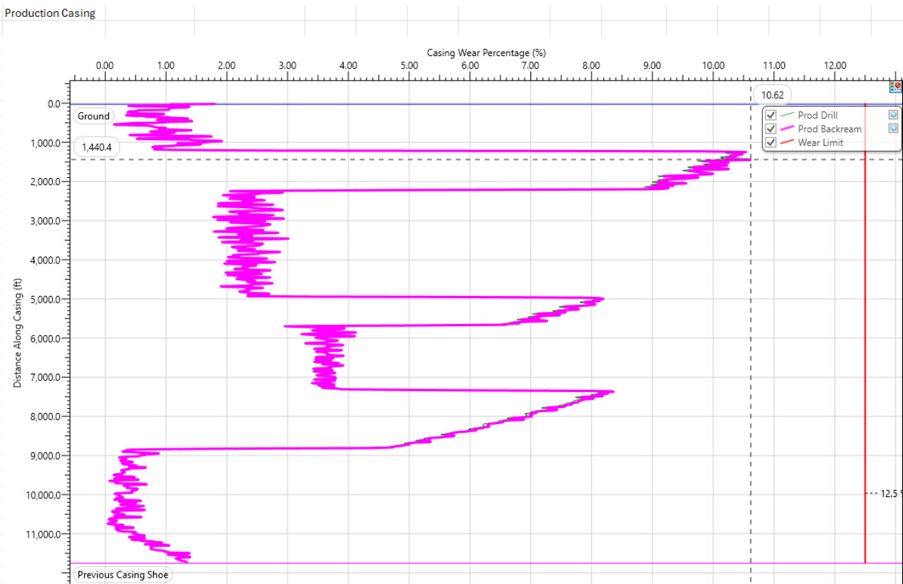
Fig. 4.3 PROD HS Casing Wear
