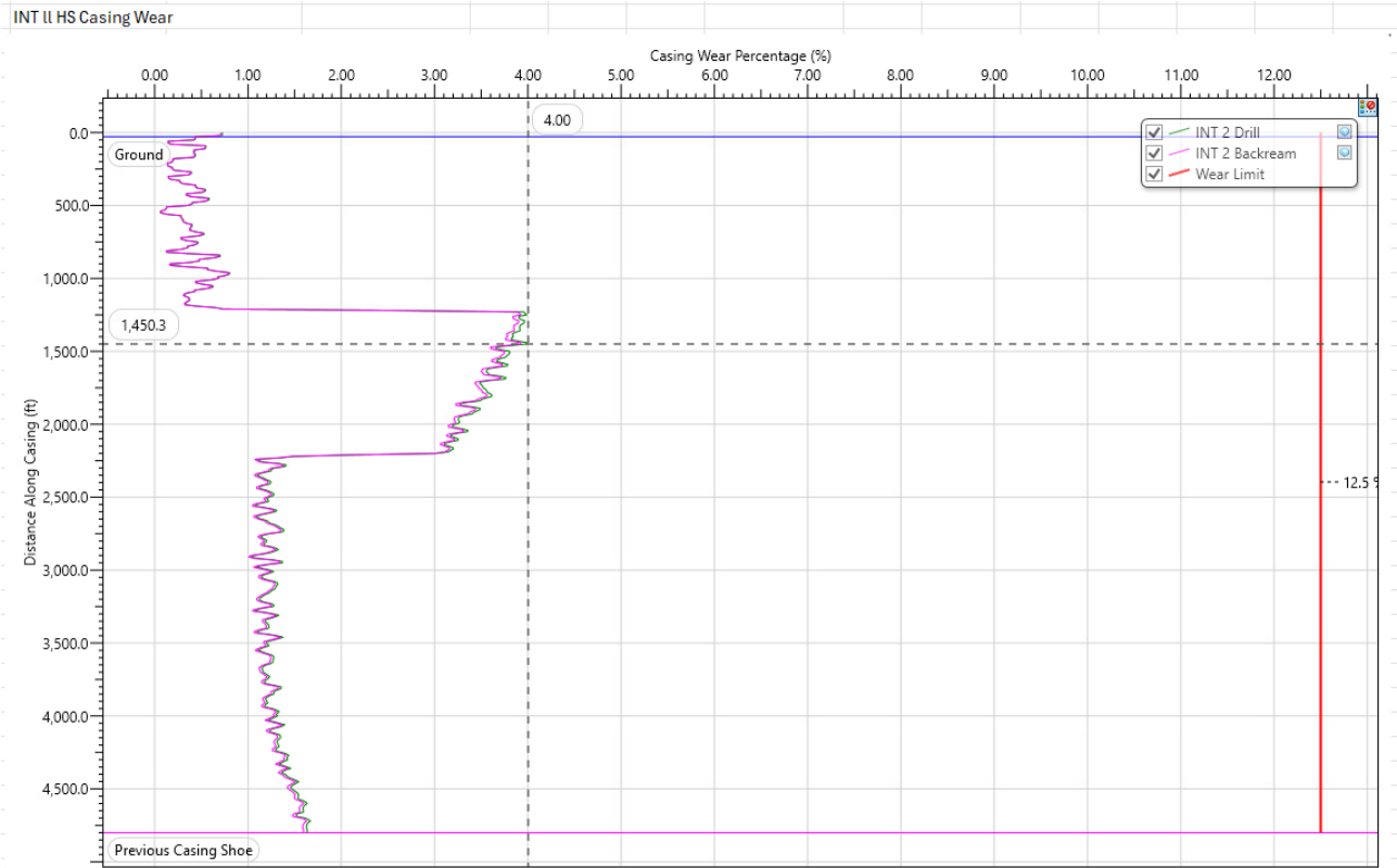
Fig. 4.2 INT2 HS Casing Wear
