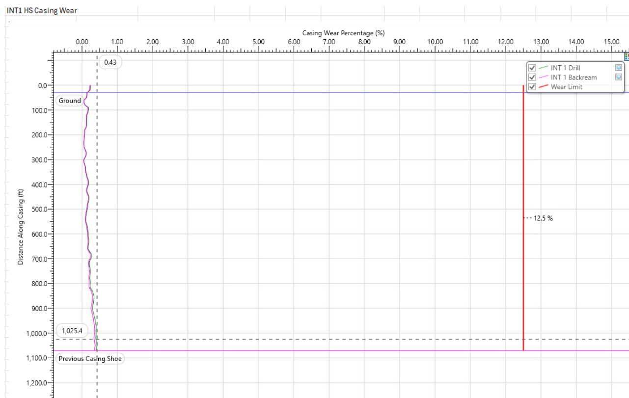
Fig. 4.1 INT1 HS Casing Wear
