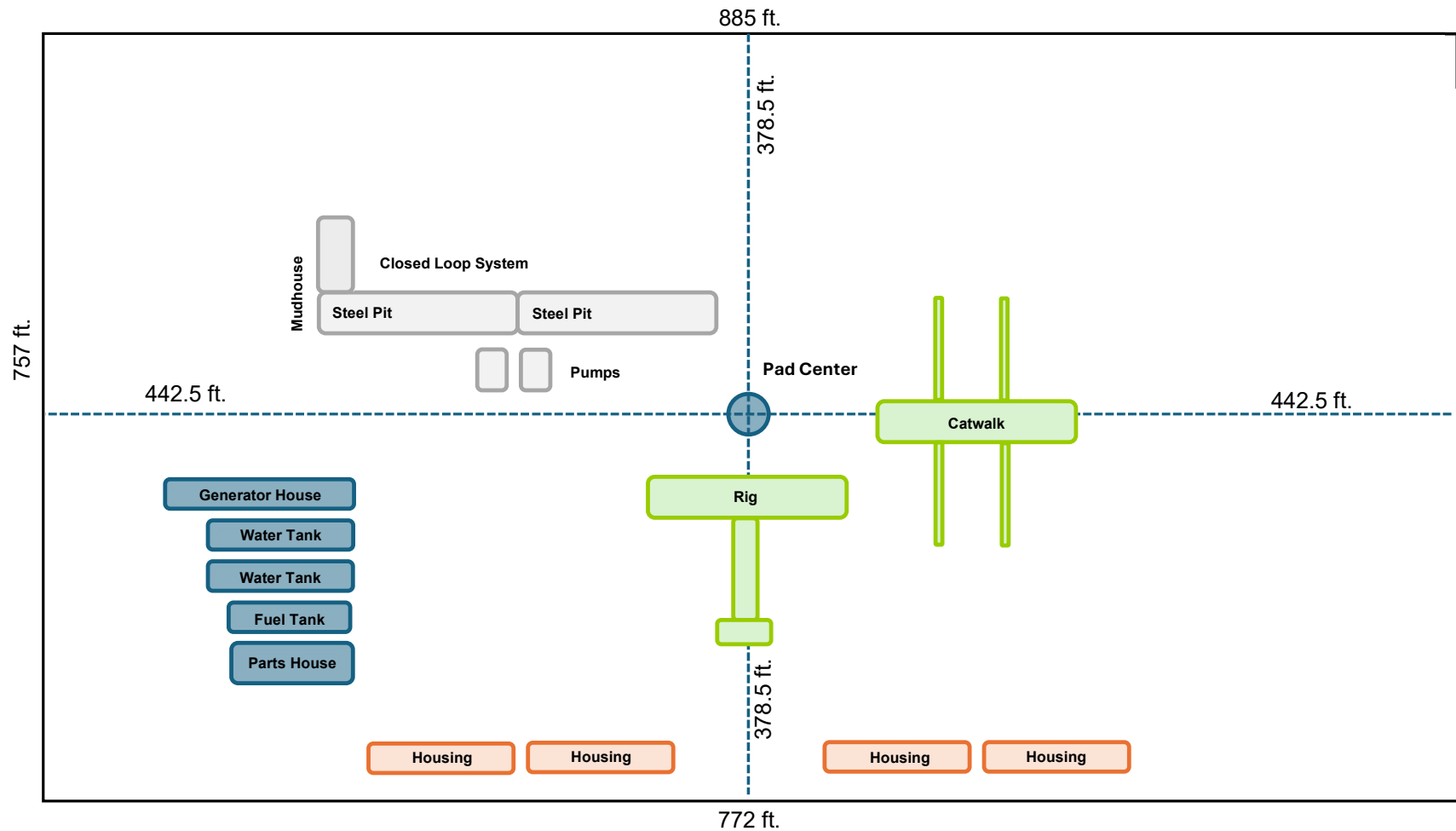
Solstice Pad 2 Rig Layout
