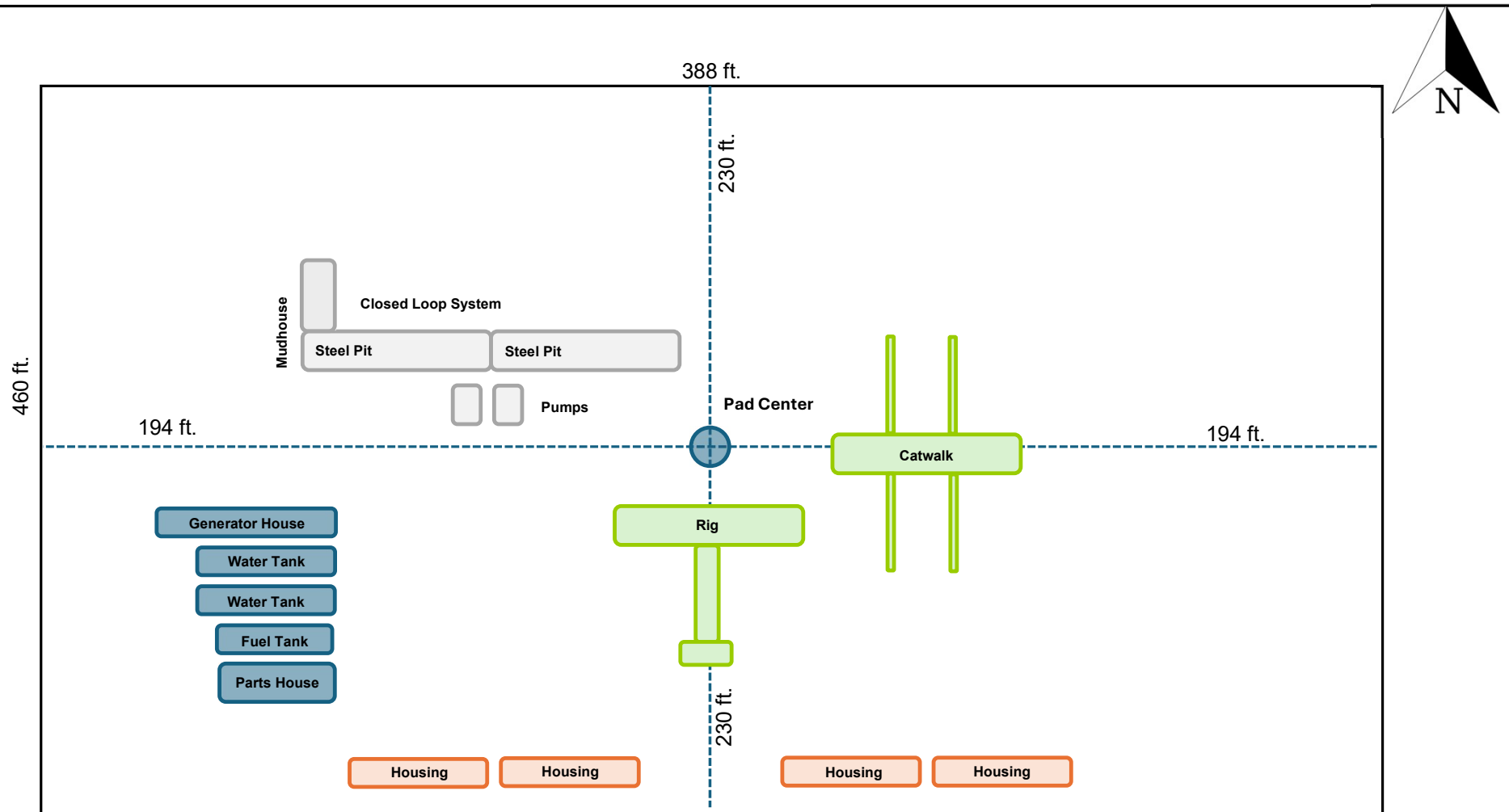
Solstice Pad 4 Rig Layout
