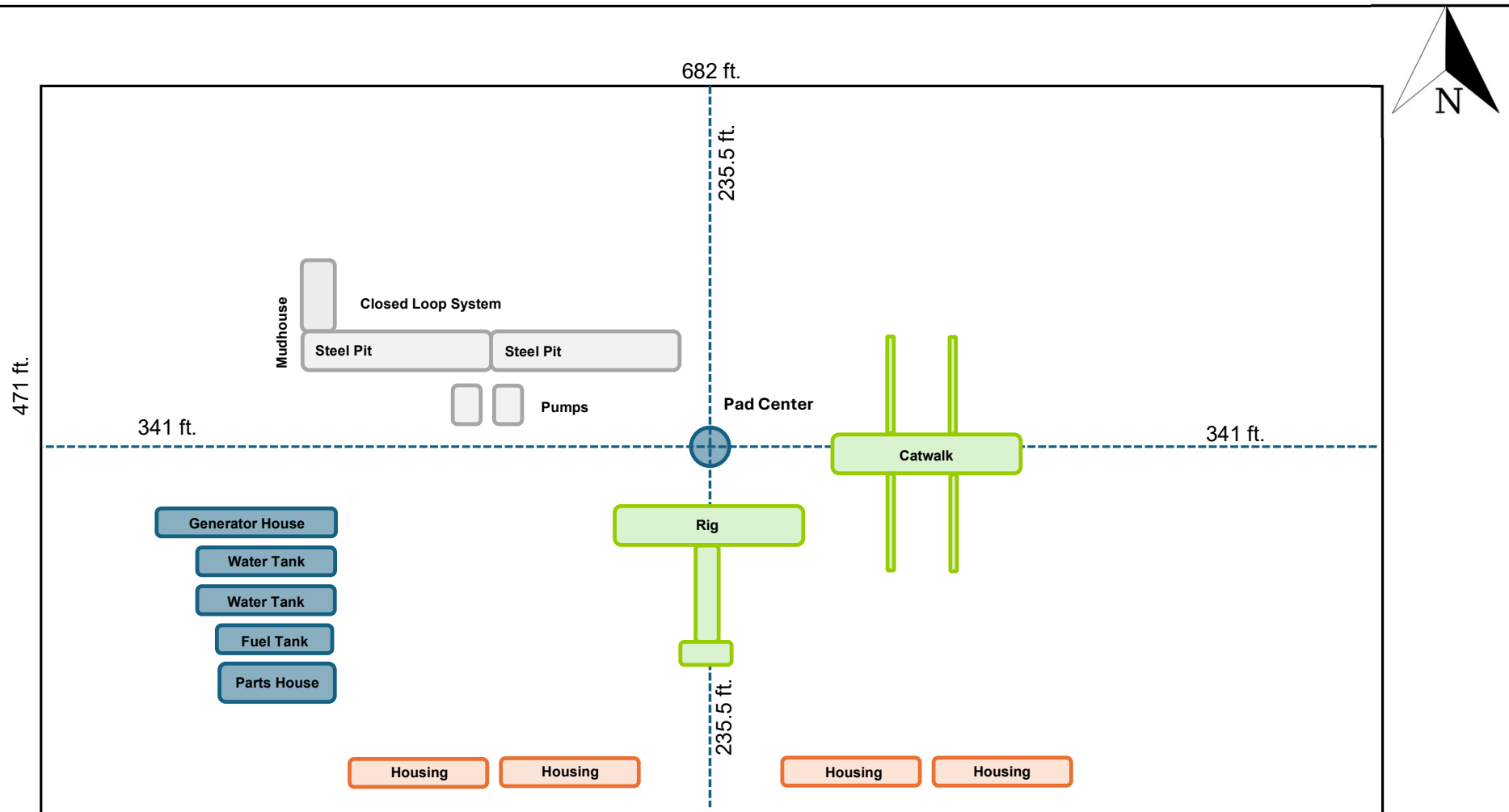
Solstice Pad 1 Rig Layout
