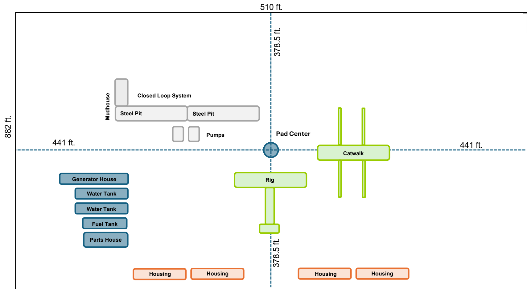
Solstice Pad 3 Rig Layout
