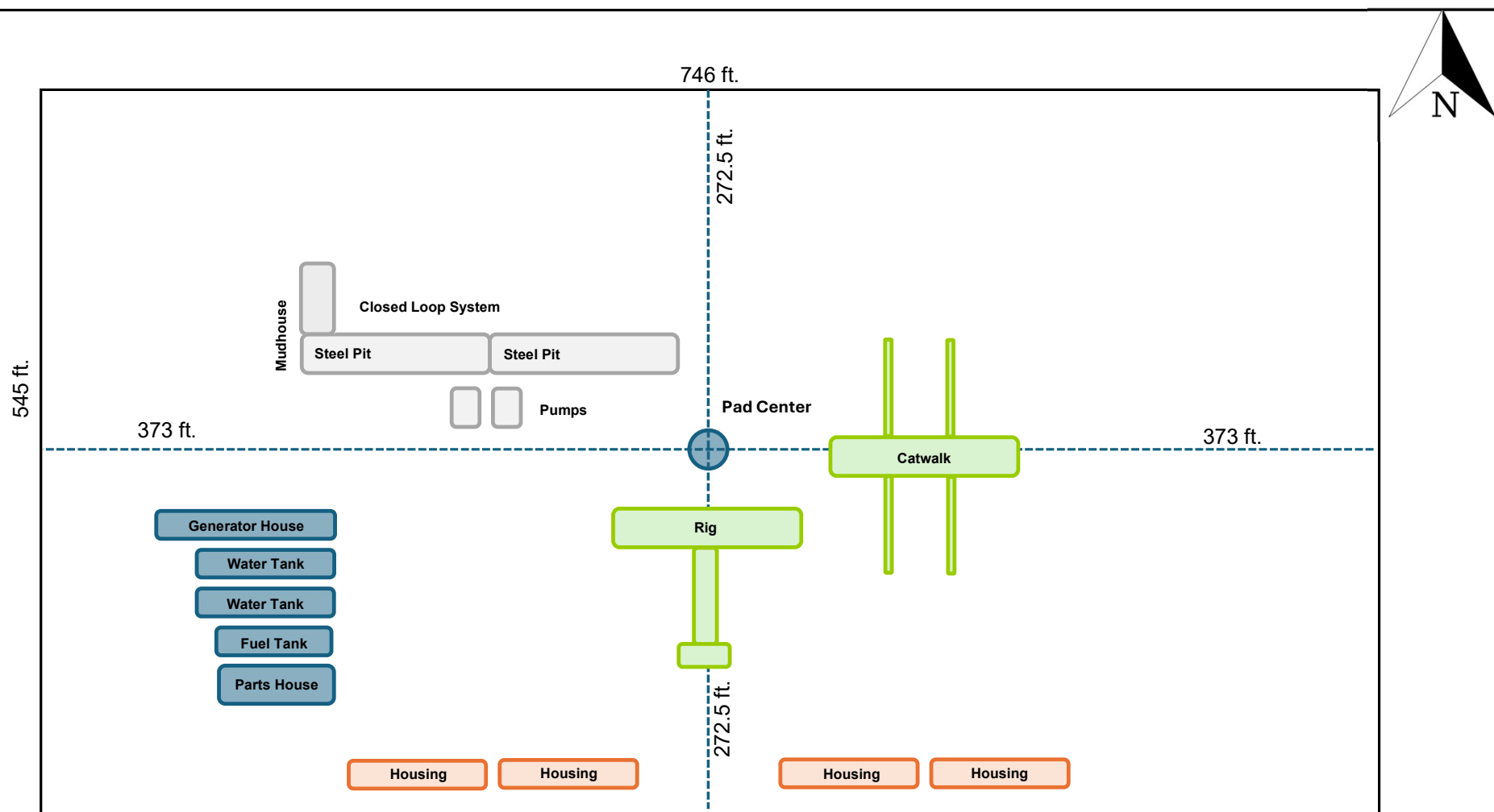
Solstice Pad 5 Rig Layout
