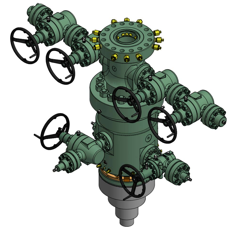
ISOMETRIC VIEW
