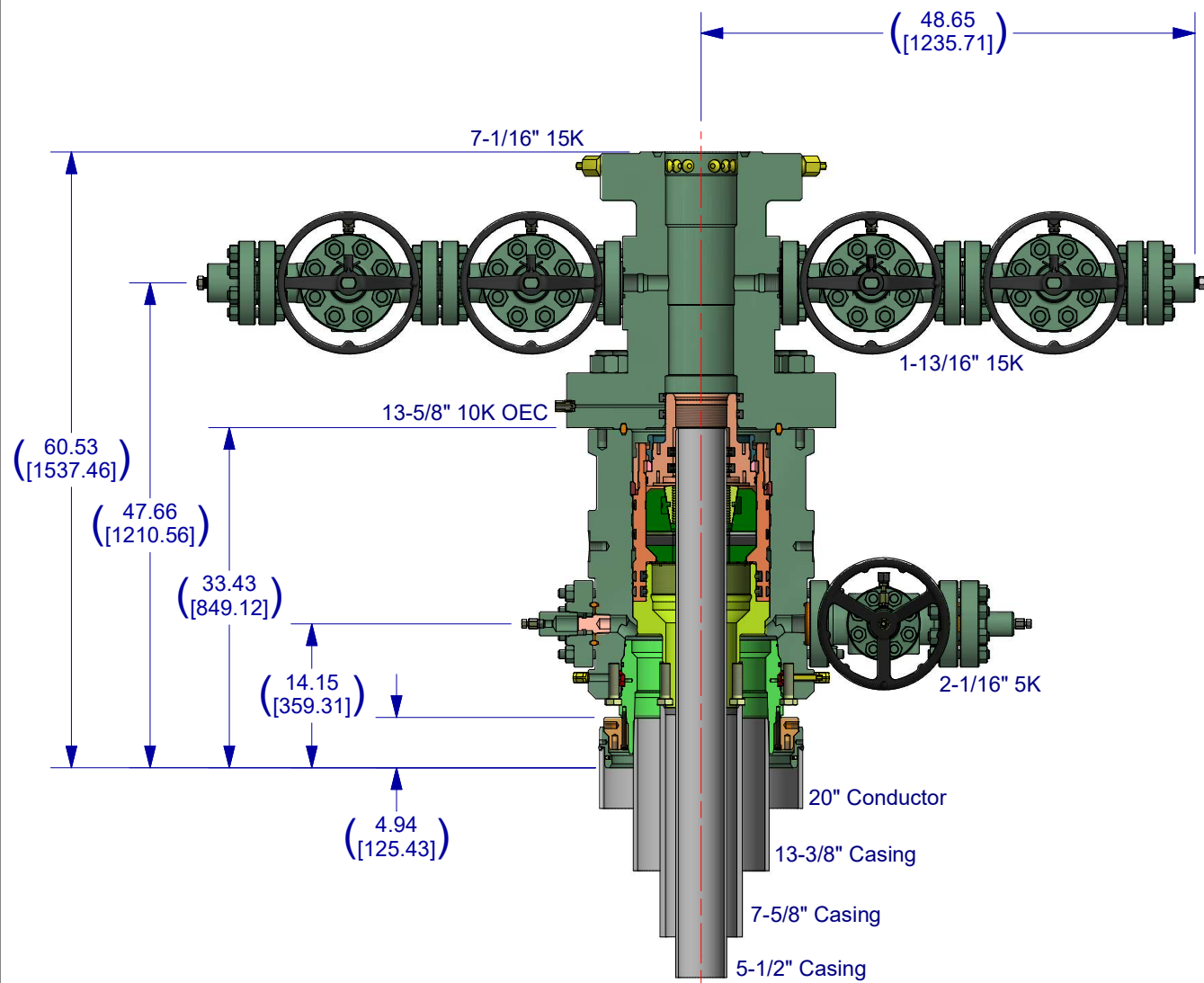
VIEW SHOWING LOWER OUTLETS
