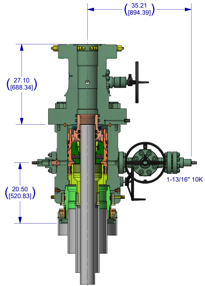
VIEW SHOWING UPPER OUTLETS
