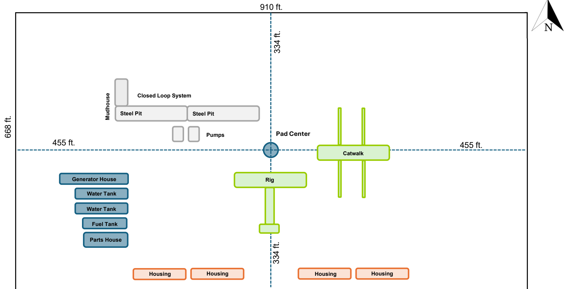
Asteroid East Pad (Expansion) Rig Layout
