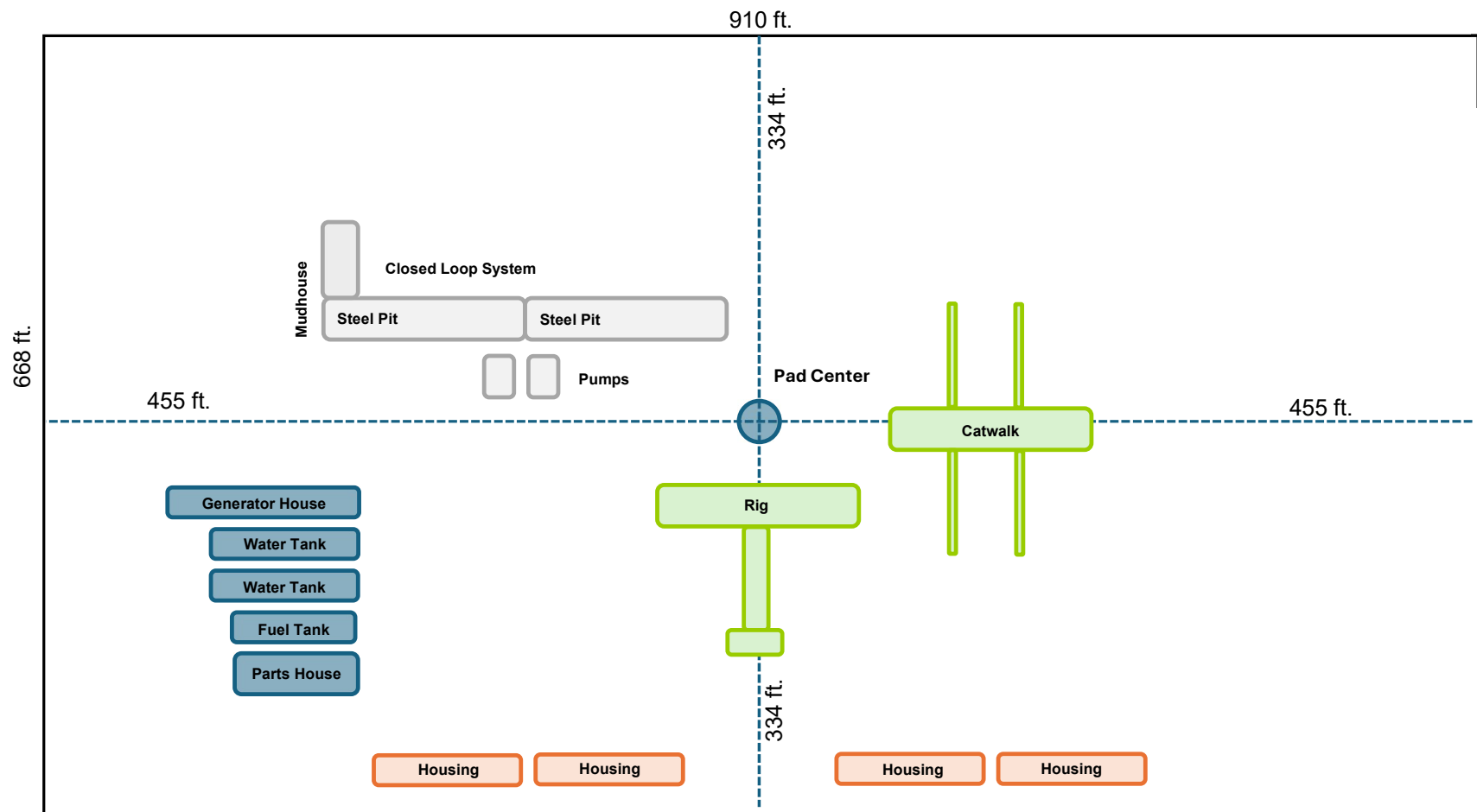
Asteroid East Pad (Expansion) Rig Layout
