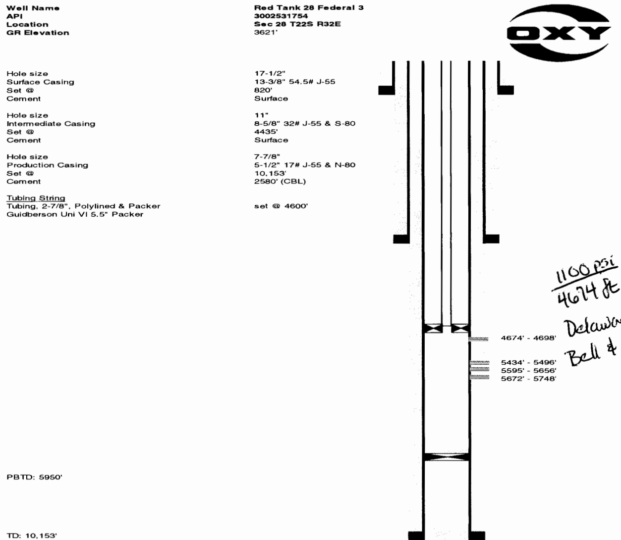
Figure 1: Red Tank 28 Federal 3 Well Schematic.
