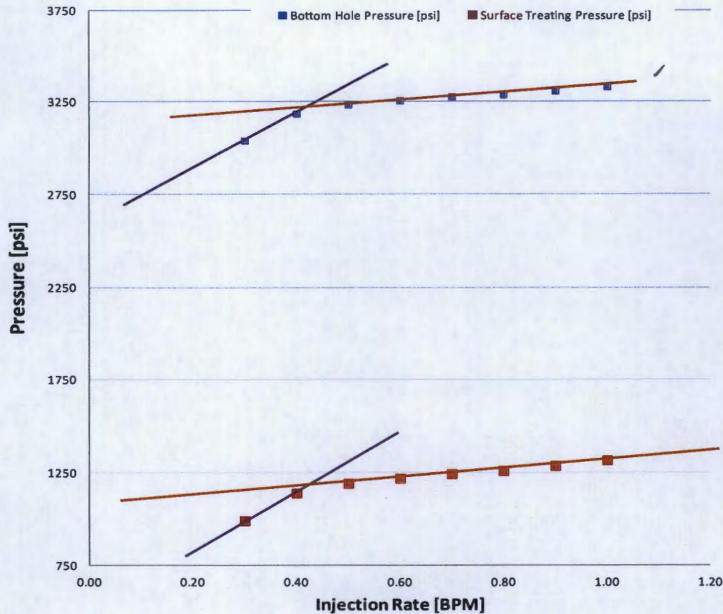
Figure 2: Surface Treating Pressure & Calculated Bottom Hole Pressure versus injection rate.
