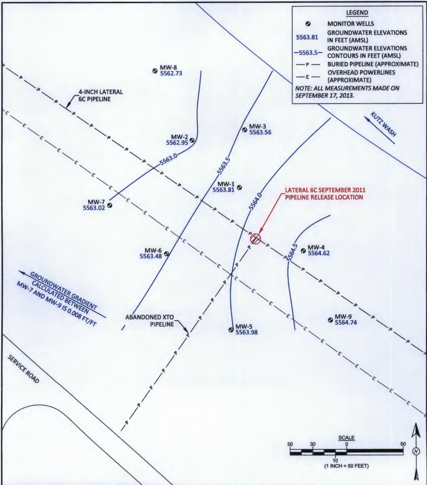
FIGURE 3 GROUNDWATER ELEVATION CONTOURS SEPTEMBER 2013 ENTERPRISE FIELD SERVICES, LLC LATERAL 6C SEPTEMBER 2011 PIPELINE RELEASE NE¼ SW¼, SECTION 26, T28N, R11W SAN JUAN COUNTY, NEW MEXICO N36.63202, W107.97400
