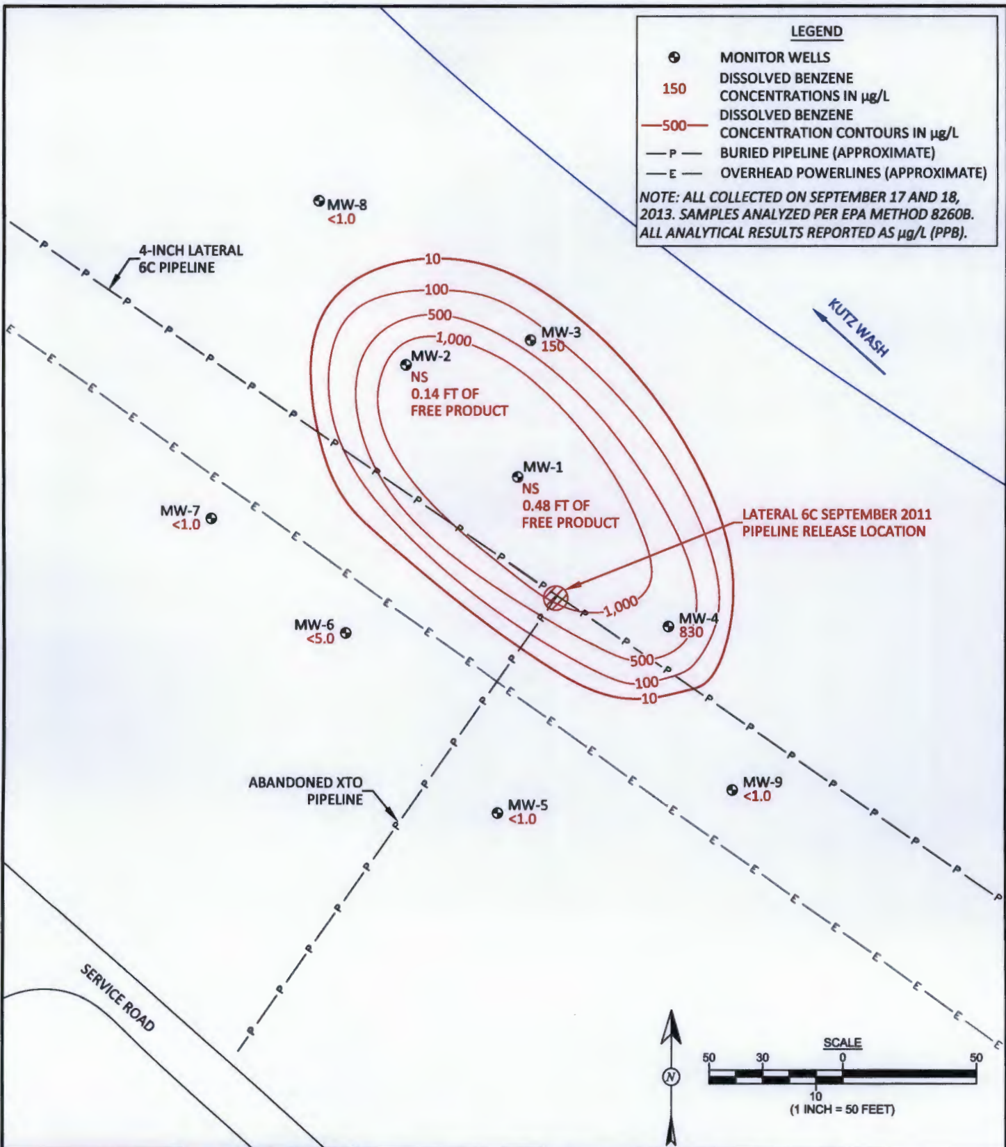
FIGURE 5 DISSOLVED BENZENE CONCENTRATION CONTOURS, SEPTEMBER 2013 ENTERPRISE FIELD SERVICES, LLC LATERAL 6C SEPTEMBER 2011 PIPELINE RELEASE NE¼ SW¼, SECTION 26, T28N, R11W SAN JUAN COUNTY, NEW MEXICO N36.63202, W107.97400
