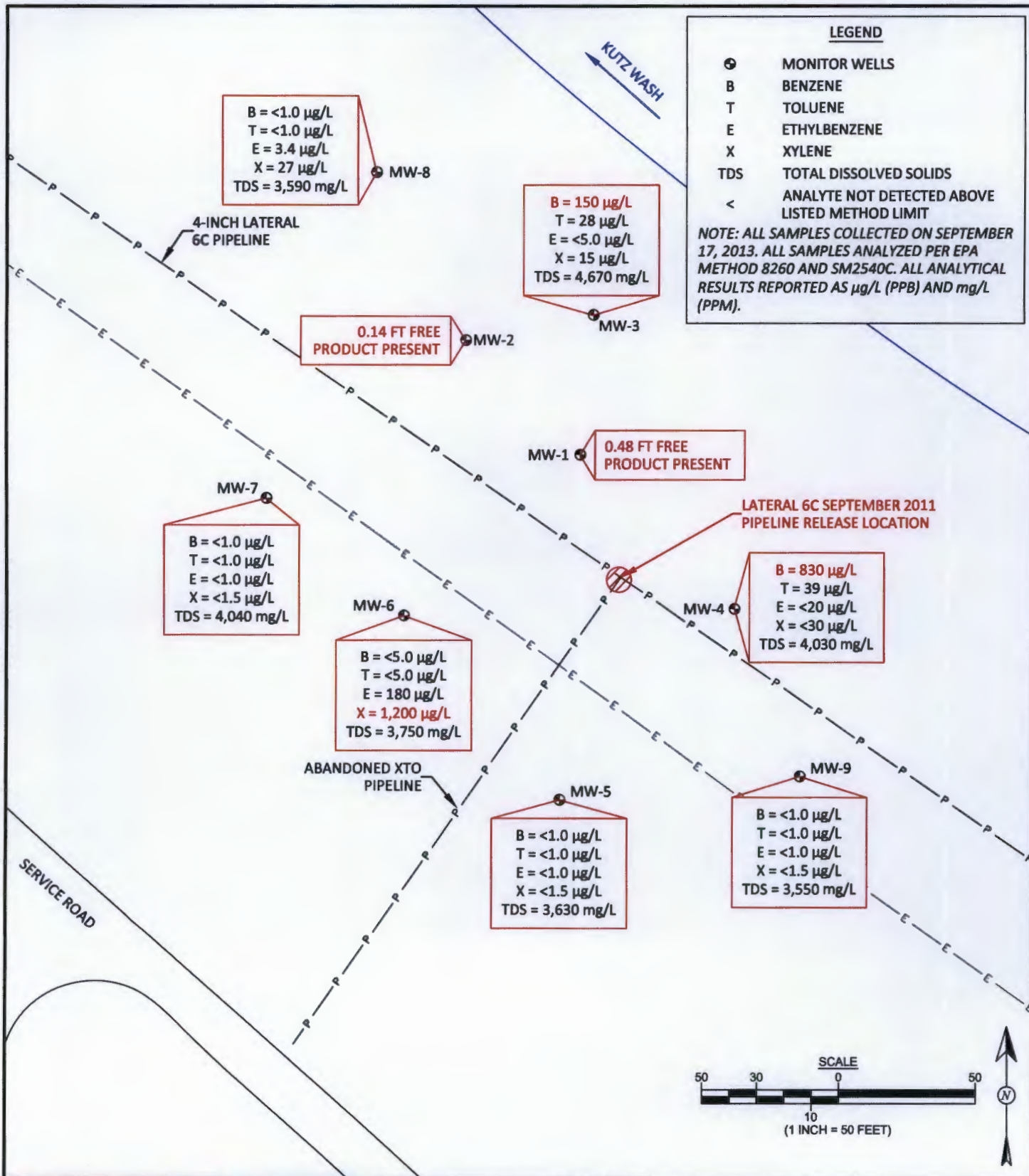
FIGURE 4 GROUNDWATER CONTAMINANT CONCENTRATIONS, SEPTEMBER 2013 ENTERPRISE FIELD SERVICES, LLC LATERAL 6C SEPTEMBER 2011 PIPELINE RELEASE NE \frac{1}{4} , SW \frac{1}{4} , SECTION 26, T28N, R11W SAN JUAN COUNTY, NEW MEXICO N36.63202, W107.97400
