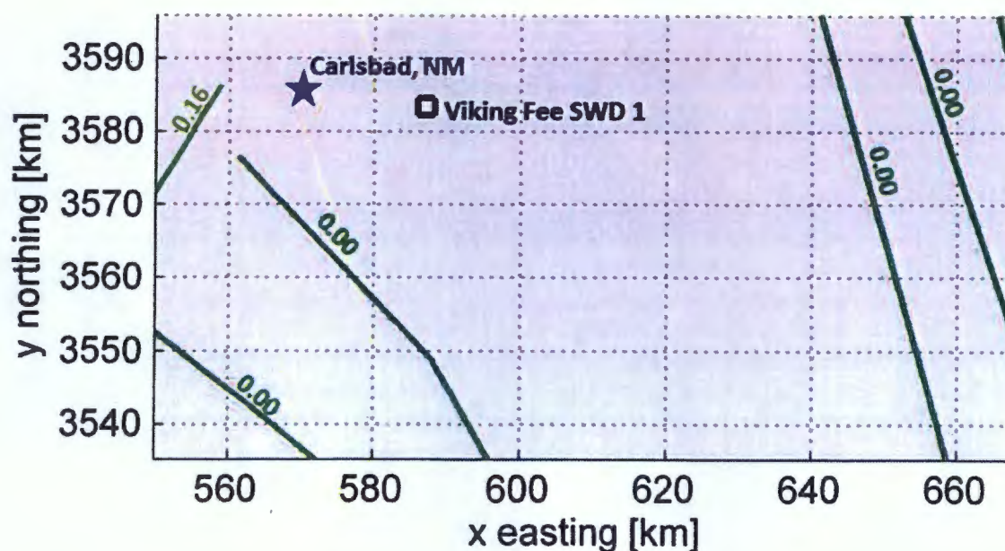
Figure 4. A map exported from the Fault Slip Potential model used in this study. Green lines indicate Precambrian fault locations. Values represent the calculated fault slip potential using the parameters indicated in Table 1.
