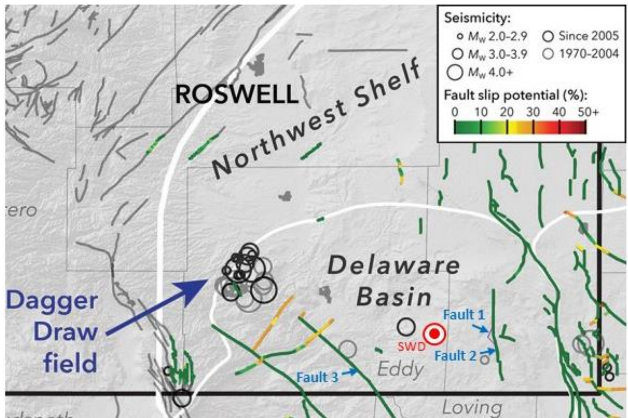
Figure 2. Modified Figure 3 from Snee and Zoback (2018). Map showing proposed location of Javelina 362330 State SWD #1 in relation to Snee and Zoback's results of their FSP analysis. Fault 1 is a fault inferred by Todd Reynolds representing NGL in NMOCD Case Nos. 20141 and 21090. This fault was not included in Snee and Zoback's (2018) models.
