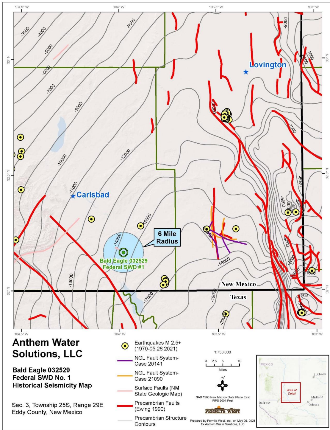
Figure 1. Structural contour map of the Precambrian basement in feet below sea level. Red lines represent the locations of Precambrian basement-penetrating faults (Ewing et al., 1990). Pink lines represent the locations of surface faults (New Mexico State Geologic Map, 2003). Purple and orange lines represent the locations of basement-penetrating faults inferred by Todd Reynolds representing NGL in NMOCD Case Nos. 20141 and 21090. The Bald Eagle 032529 Federal SWD #1 well lies ~8.3 miles northeast of the closest deeply penetrating fault and ~9.5 miles southwest of the closest historic earthquake.
