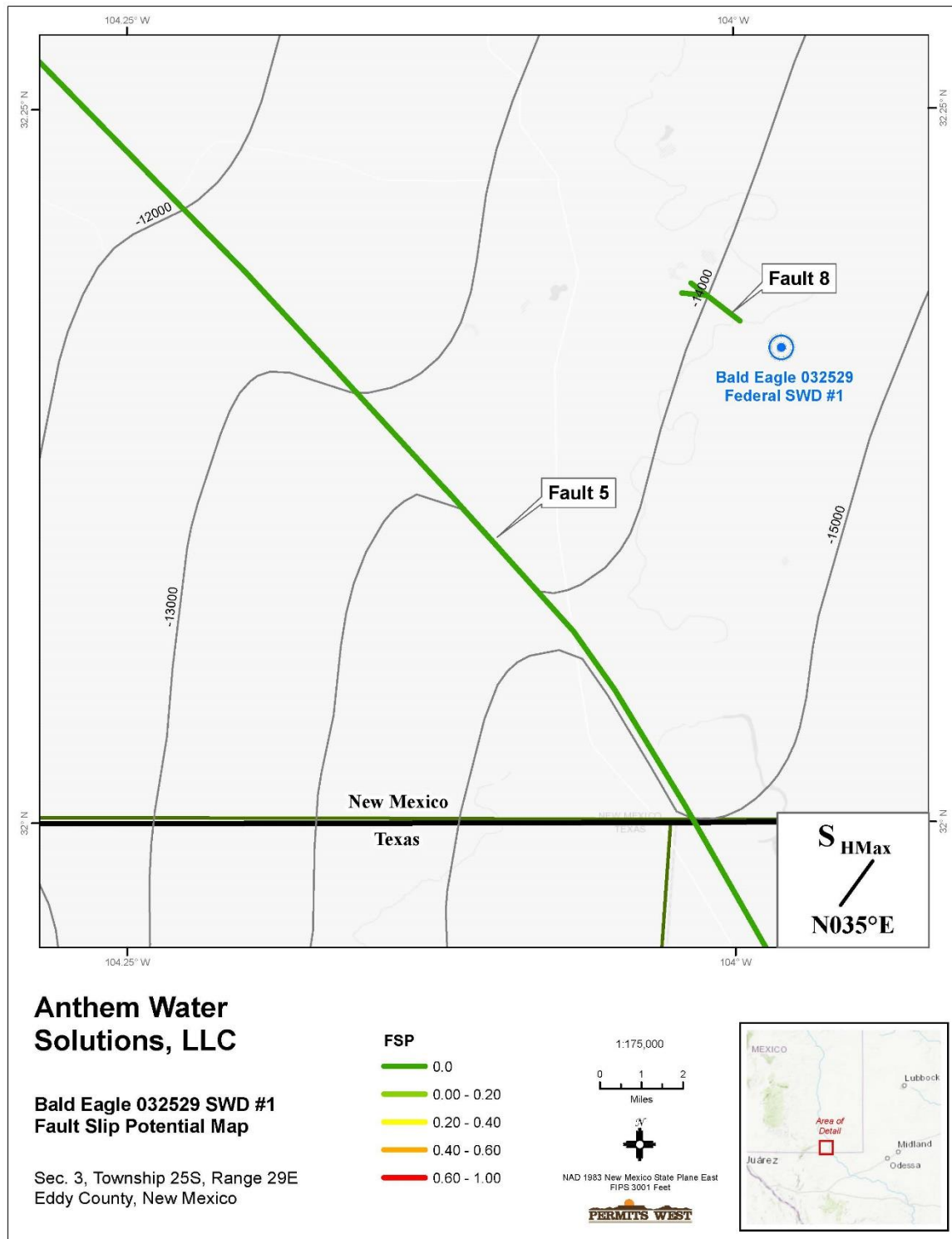
Figure 2. Fault map. Faults are colored based on probability of fault slip as modeled using Fault Slip Potential software (Walsh and Zoback, 2016). Labeled values represent the calculated fault slip potential using the parameters indicated in Table 2. Contours show the top of the Precambrian basement in feet below sea level.
