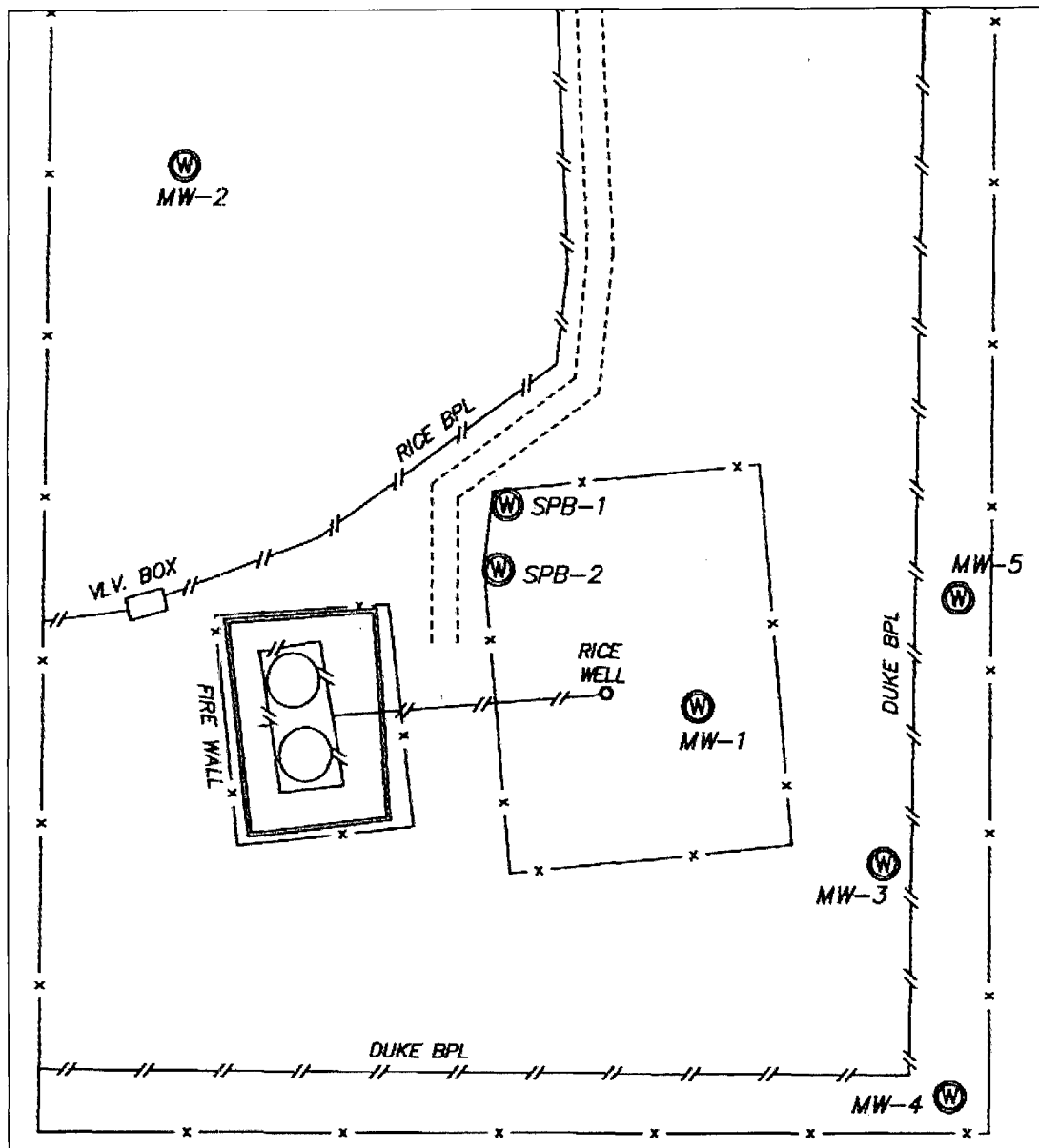
EME H-20 SWD monitor well and bio-sparg well locations.
