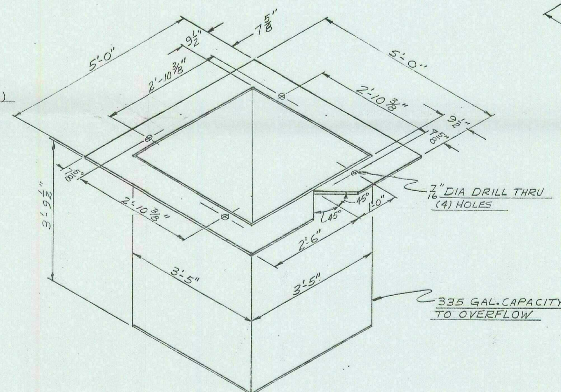
LINER WELDED CONSTR. 10 GA. (.134)
