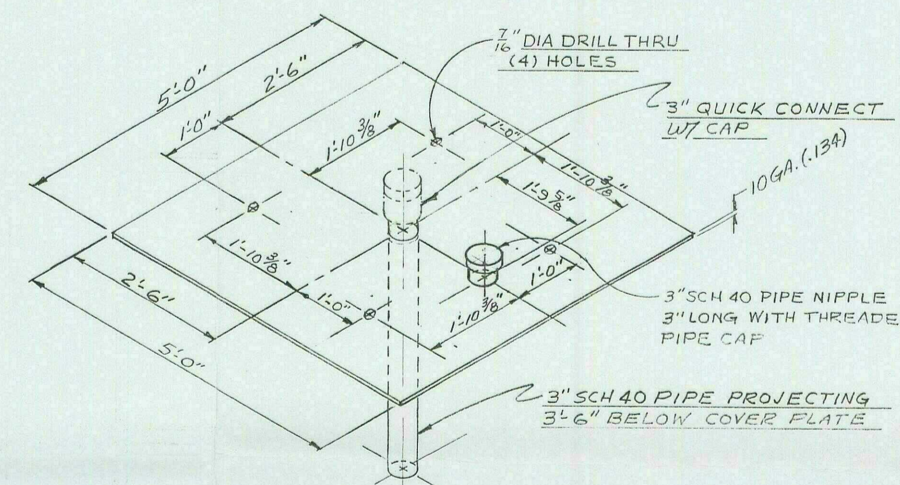
SUMP COVER PLATE WELDED CONSTR. C.S.
