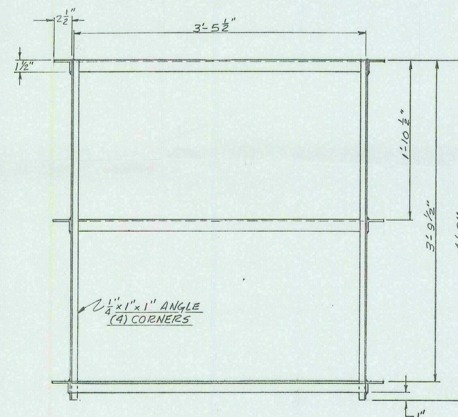
SECTION "A-A" WELDED CONSTR.
