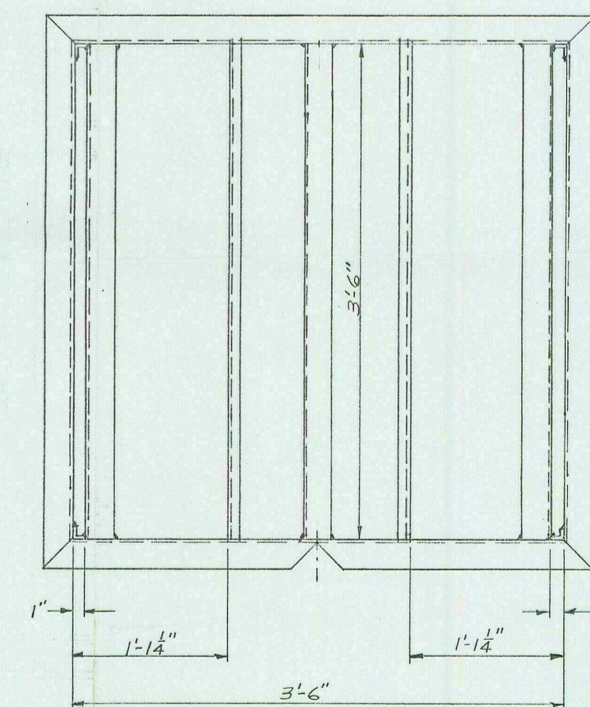
SECTION "B-B" WELDED CONSTR. C.S.
