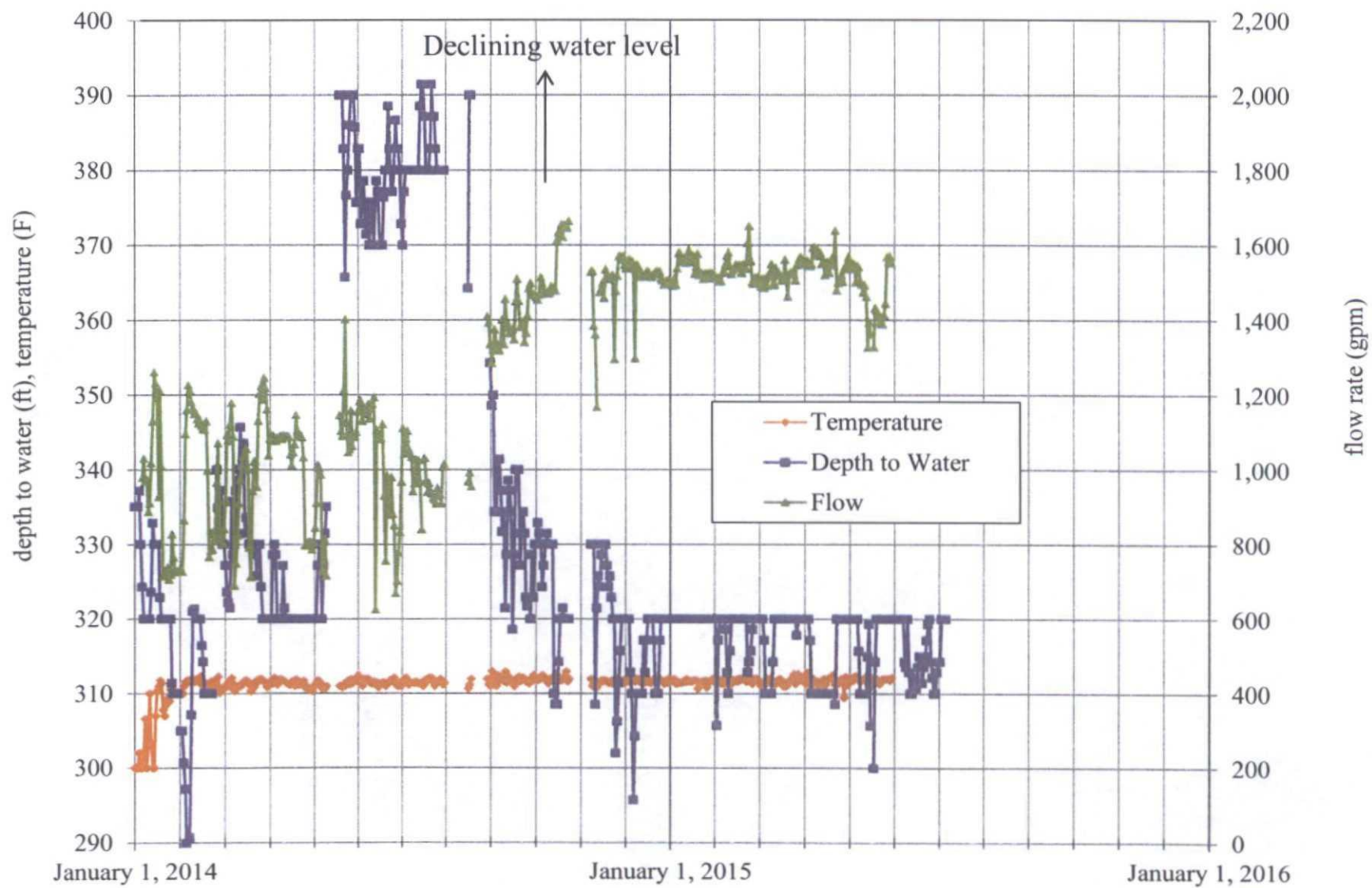
Temperature, Depth to Water, and Flow Rate, Production Well 45-7
