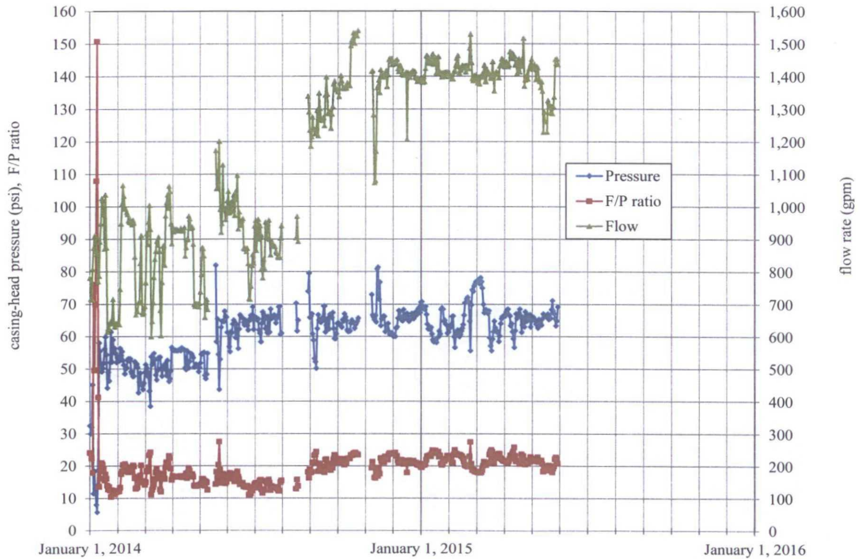
Casing-head Pressure and Flow Rate, Injection Well 55-7
