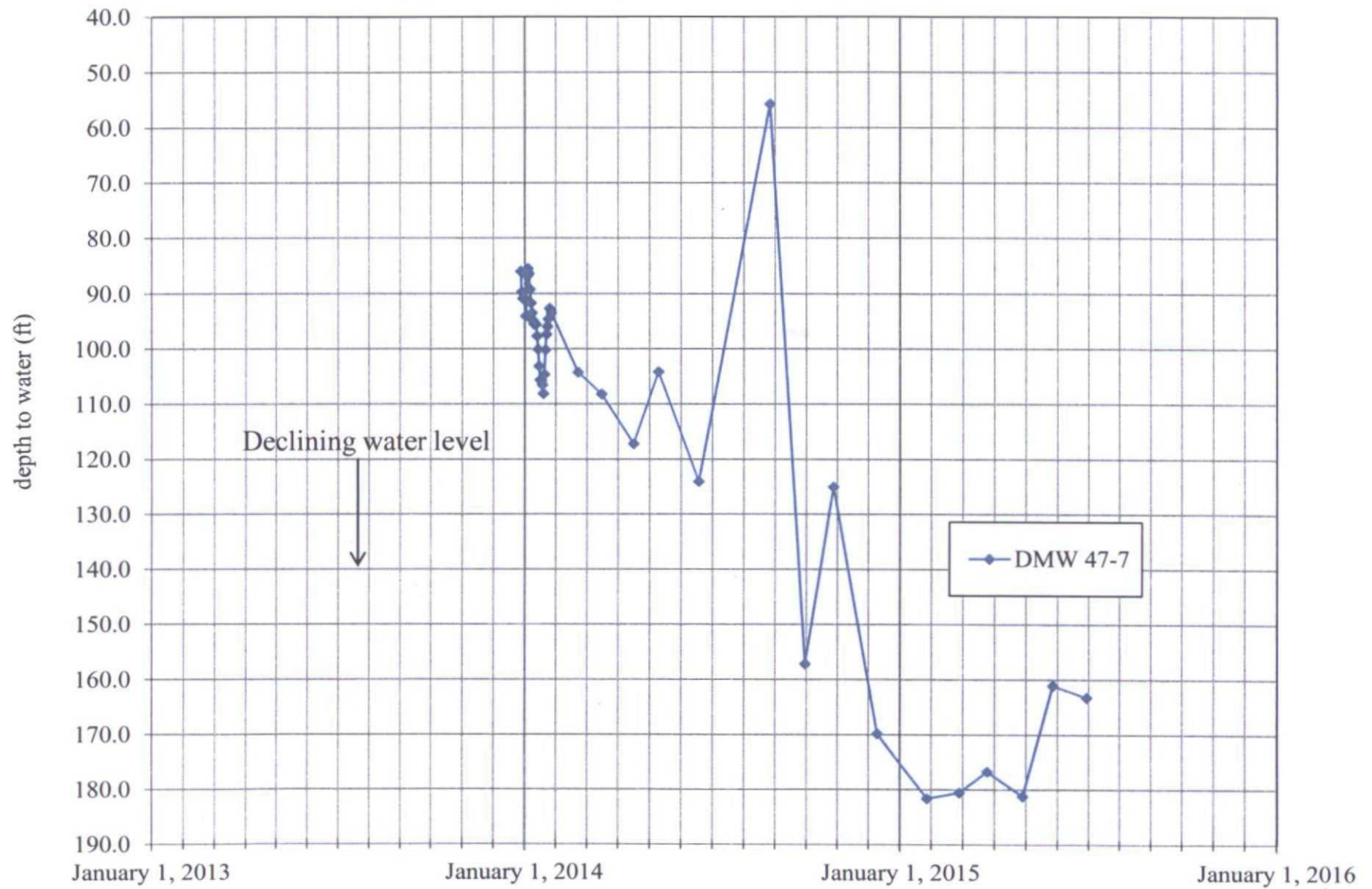
Depth to Water, Deep Monitoring Well DMW 47-7
