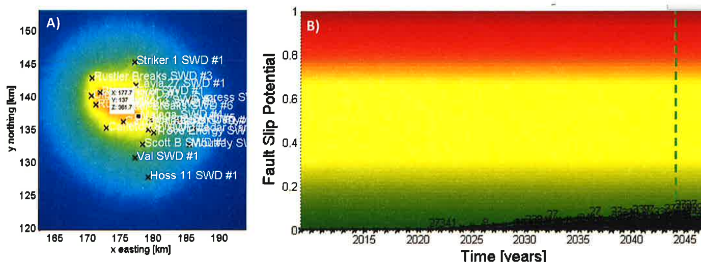
Figure 1: A) Modeled reservoir pressure for the 20 well case at year 2045. A maximum pressure of ~362 psi is observed at Malaga SWD #4. B) Fault slip potential (FSP) for the 20 well case. On all faults, FSP remains below 10%. The green dashed line marks year 2045, the black lines and numbers denote the slip probability of individual faults.
