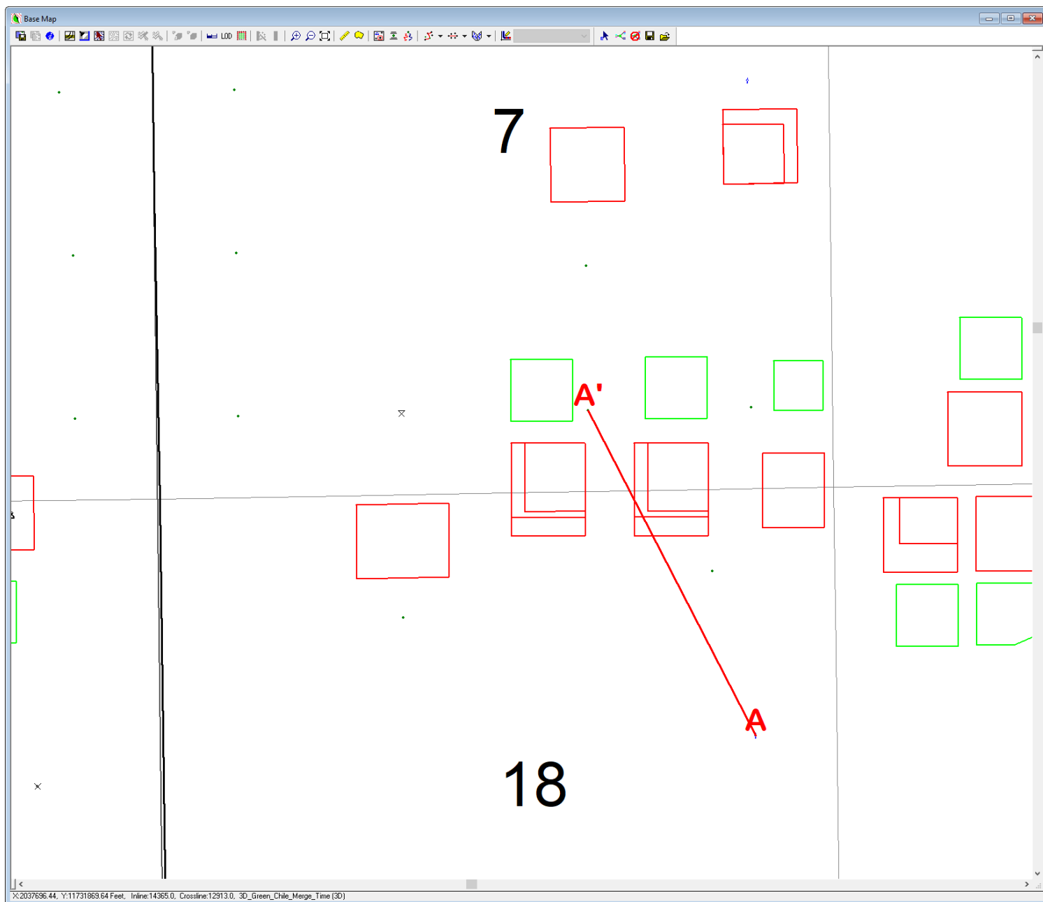
Devon Exhibit B-2 – Map showing the location of cross section A – A’.
