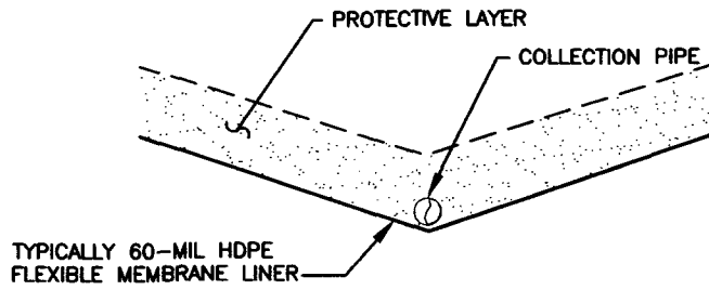
1. SINGLE LINER WITH LEACHATE COLLECTION
