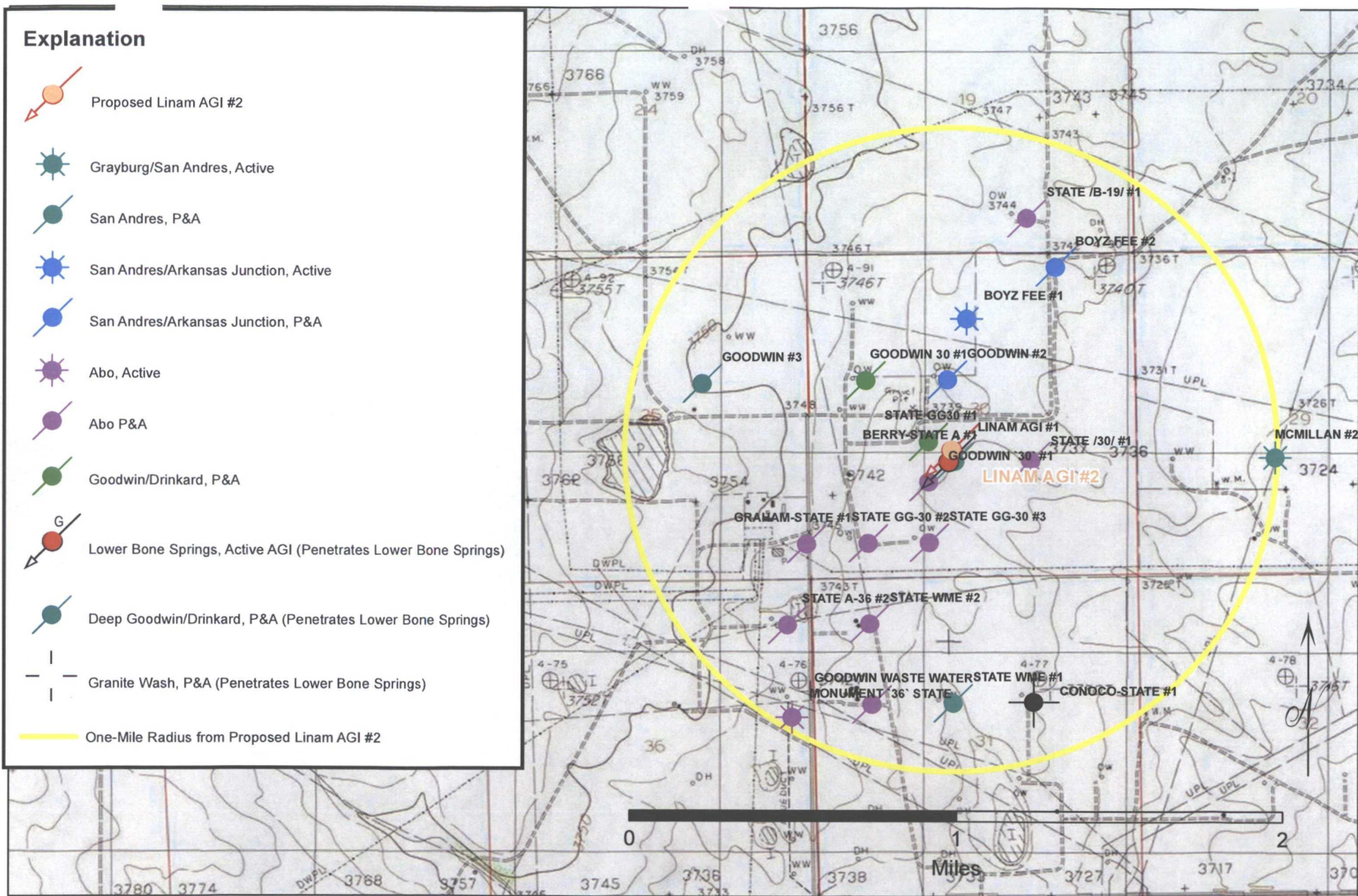
Figure 8: Oil, Gas and AGI Wells Within One Mile Radius of Proposed Linam AGI #2
