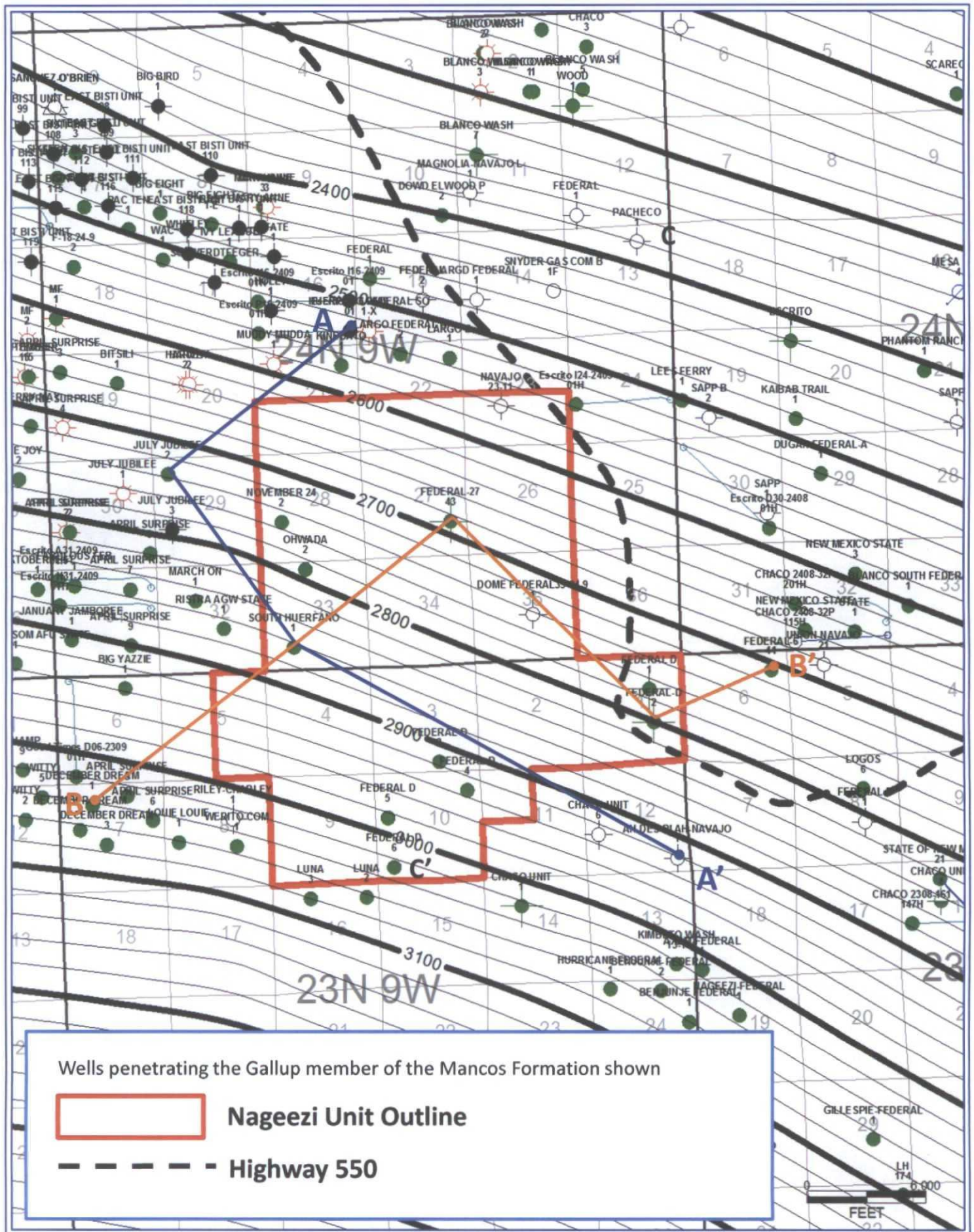
Top Mancos Structure Contour Map Sub-Sea True-Vertical Depth
