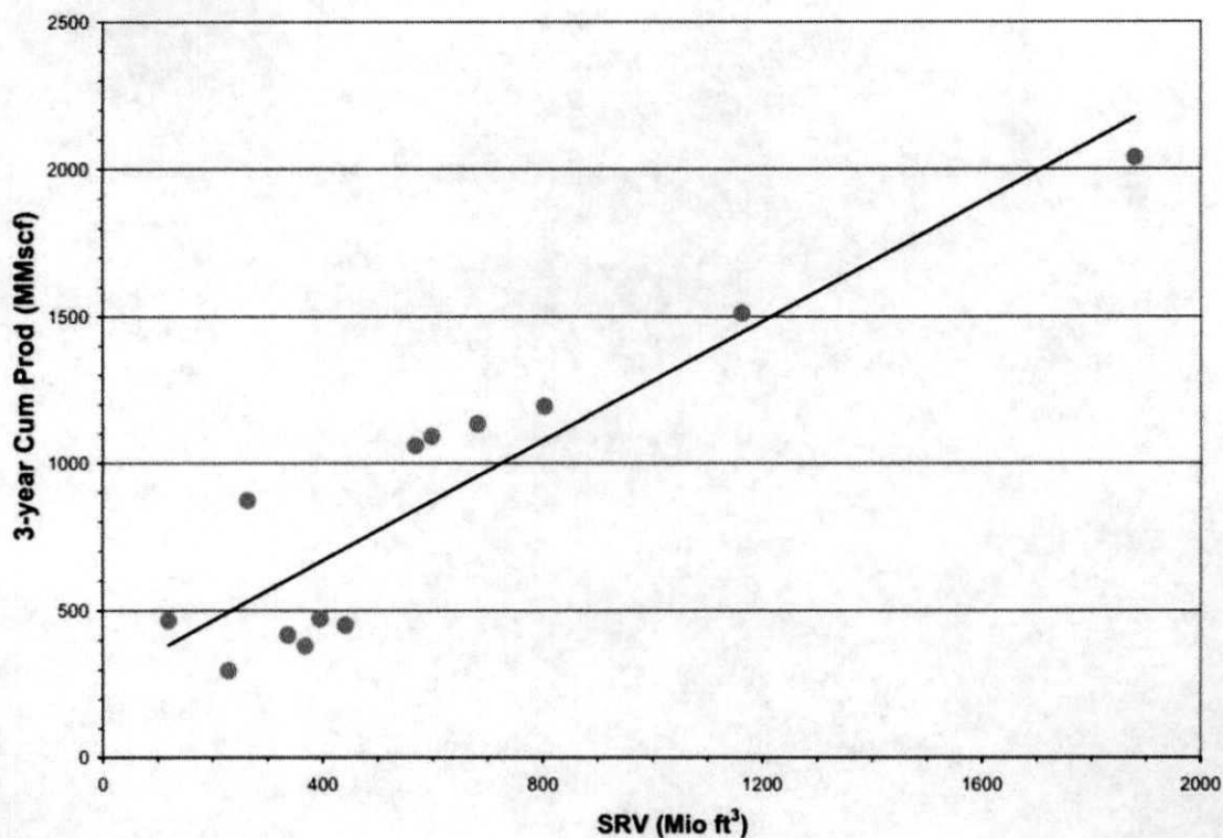
Fig. 9—SRV trend vs. 3-year cumulative horizontal-well production for one Barnett-shale county.
