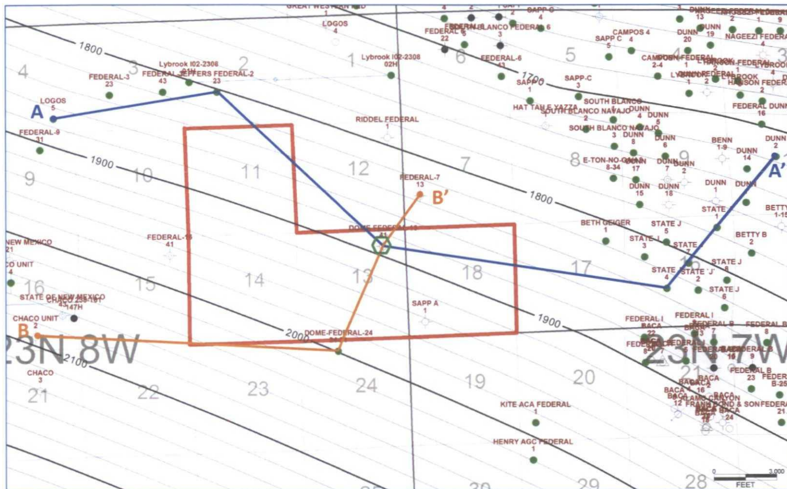
Top Gallup Structure Contour Map Sub-Sea True Vertical Depth
