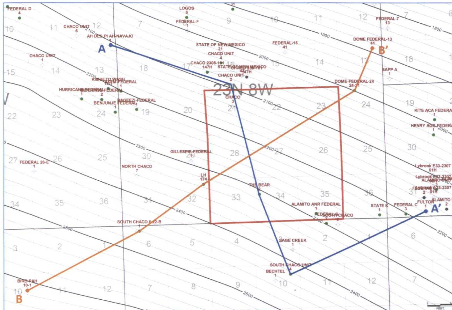
Top Gallup Structure Contour Map Sub-Sea True Vertical Depth
