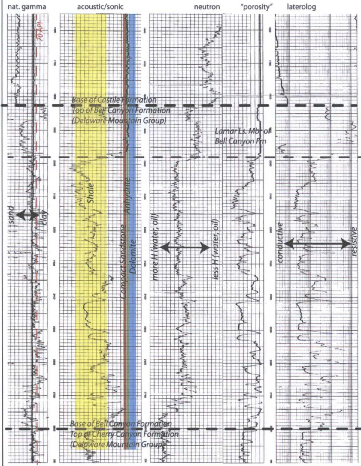
Figure 1 Log for Bell Canyon Formation Section in Section 35, T22S, R26E, Airport Grace #1 (API 30-015-20829)
