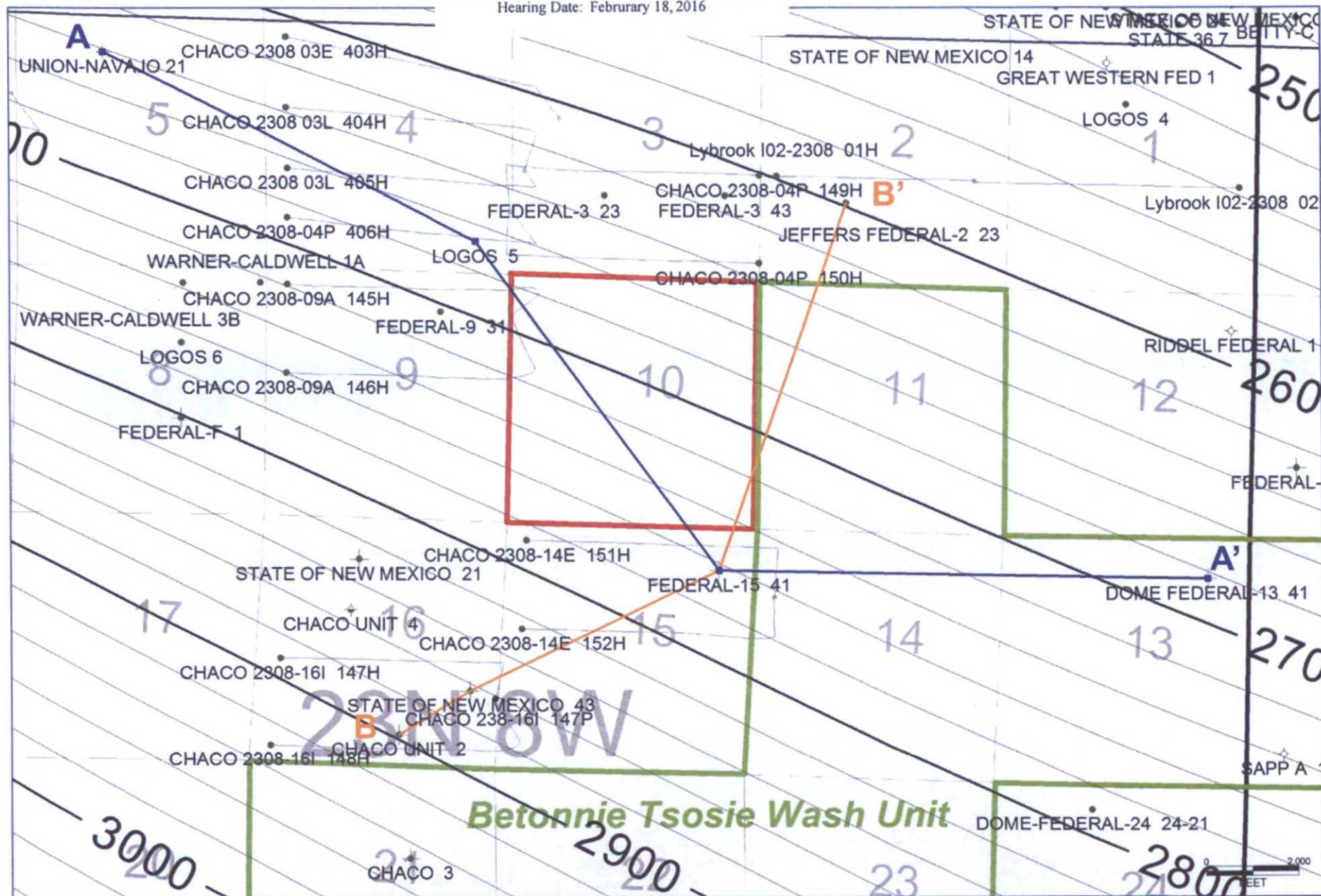
Structure contour map on top of the Mancos Shale, showing the proposed non-standard project area outlined in red (Section 10, T23N, R8W). Contour Interval = 20 feet
