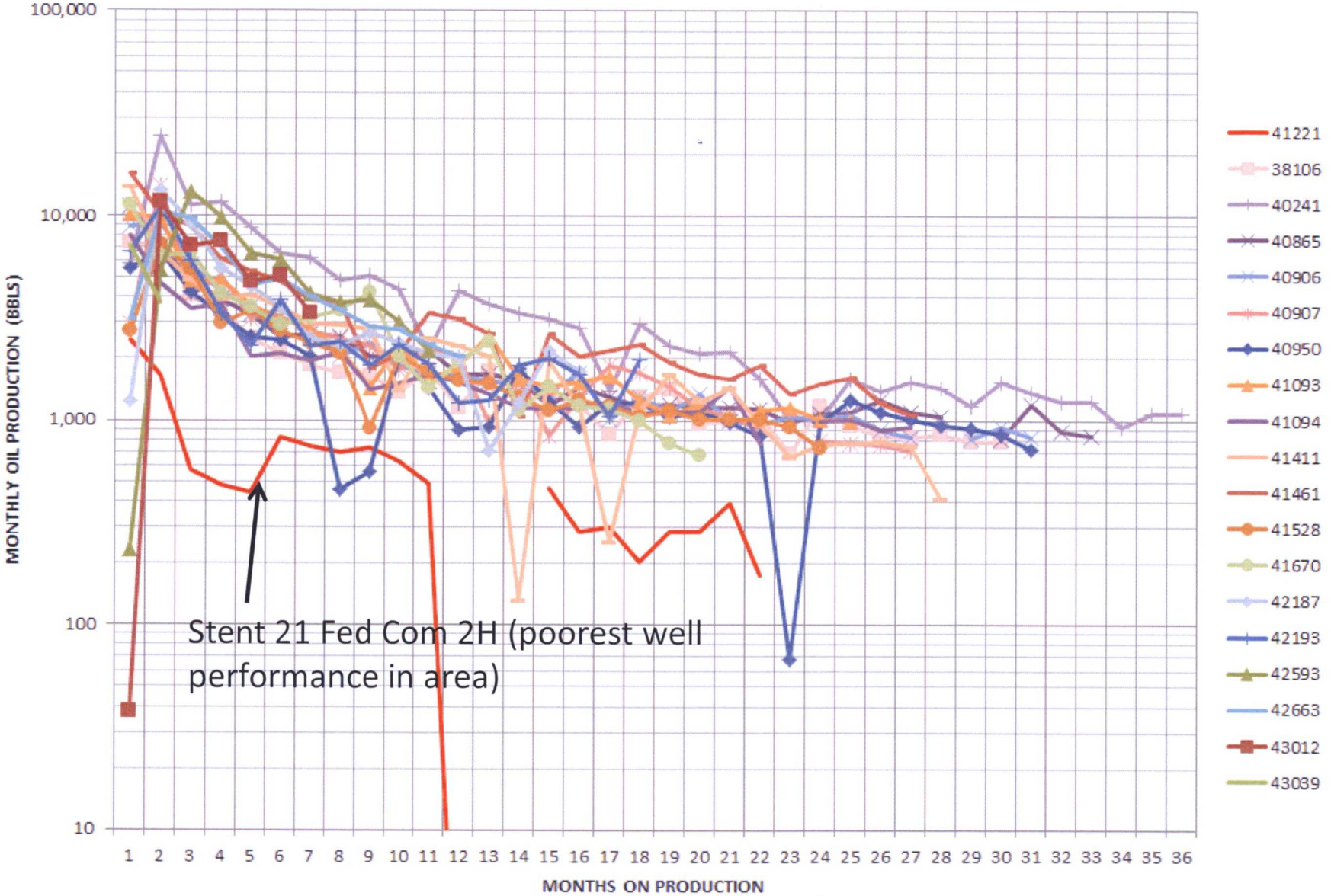
HZ WELL NORMALIZED OIL PRODUCTION - BONE SPRINGS 2 FORMATION
