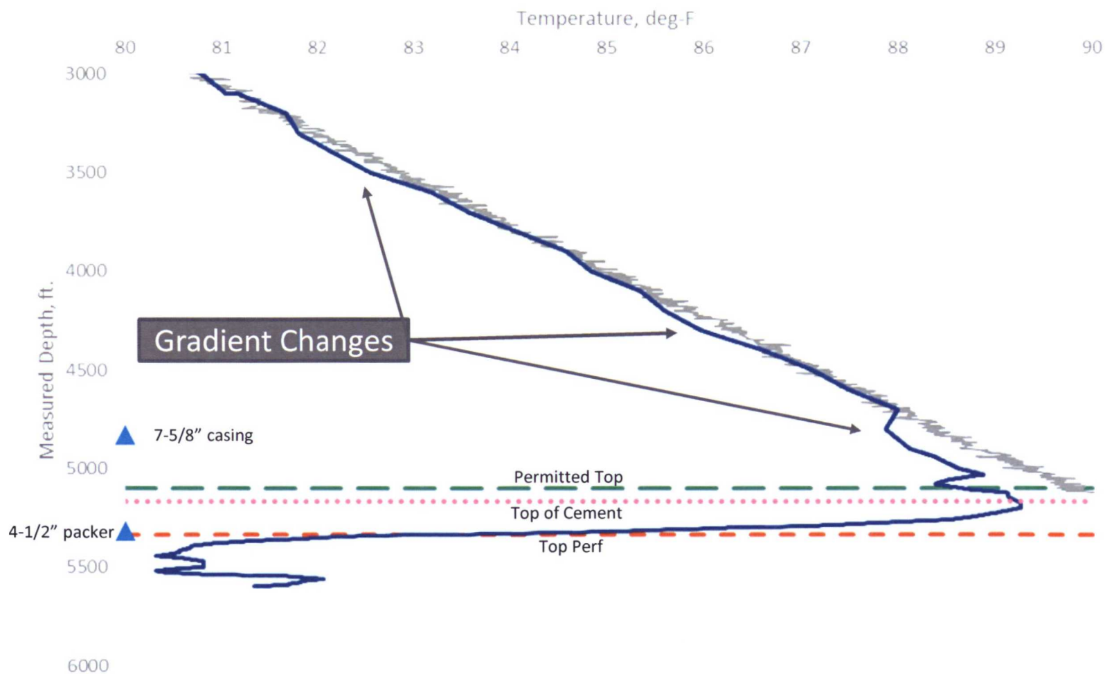
OXY - SWD Log vs. Devon offset baseline Log
