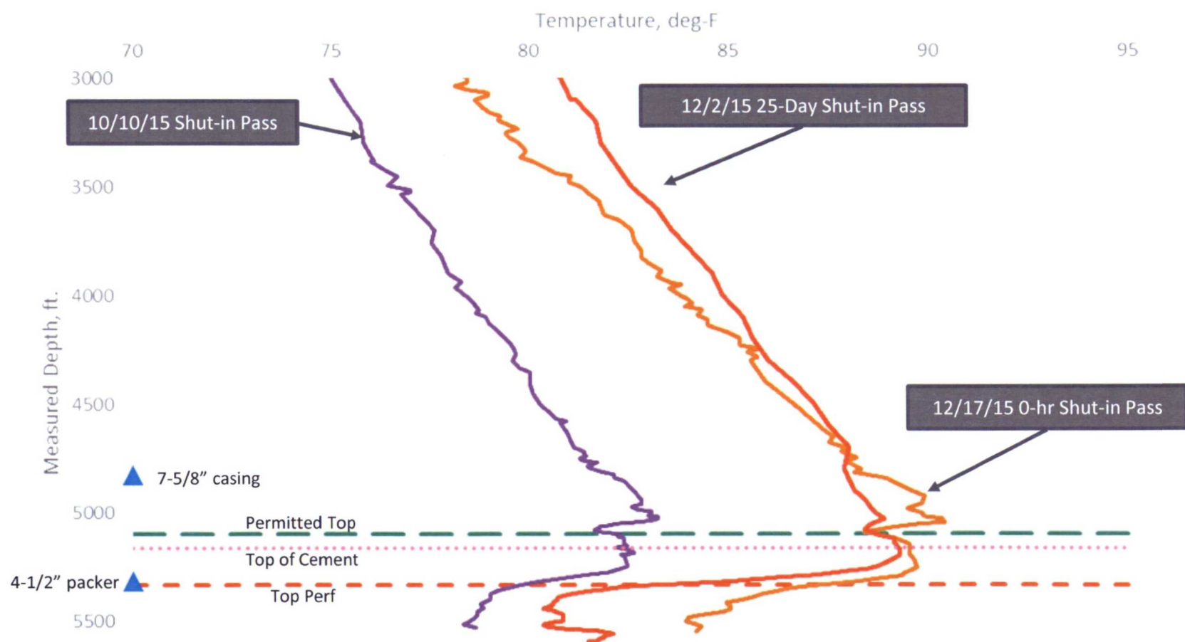
OXY - Diamond 34 State 1 SWD Temperature Logs
