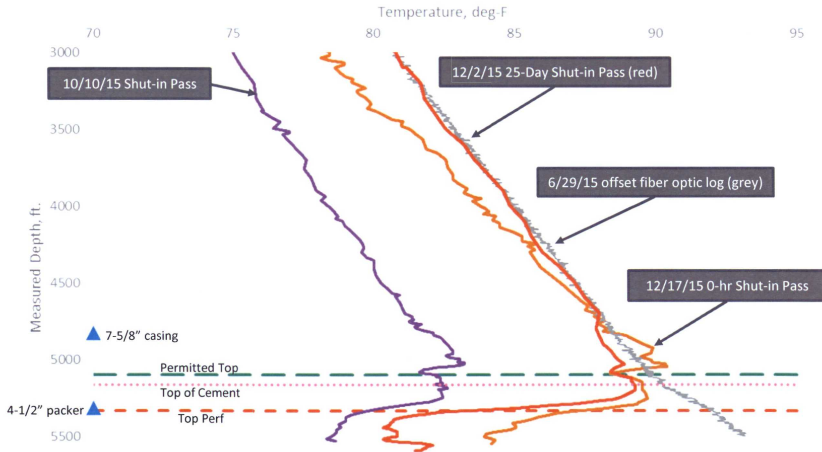
OXY - Diamond 34 State 1 SWD Temperature Logs
