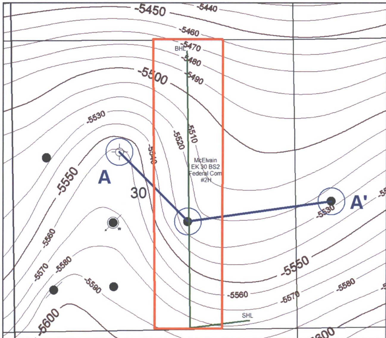
Structure map on the top of the 2nd Bone Spring sand
