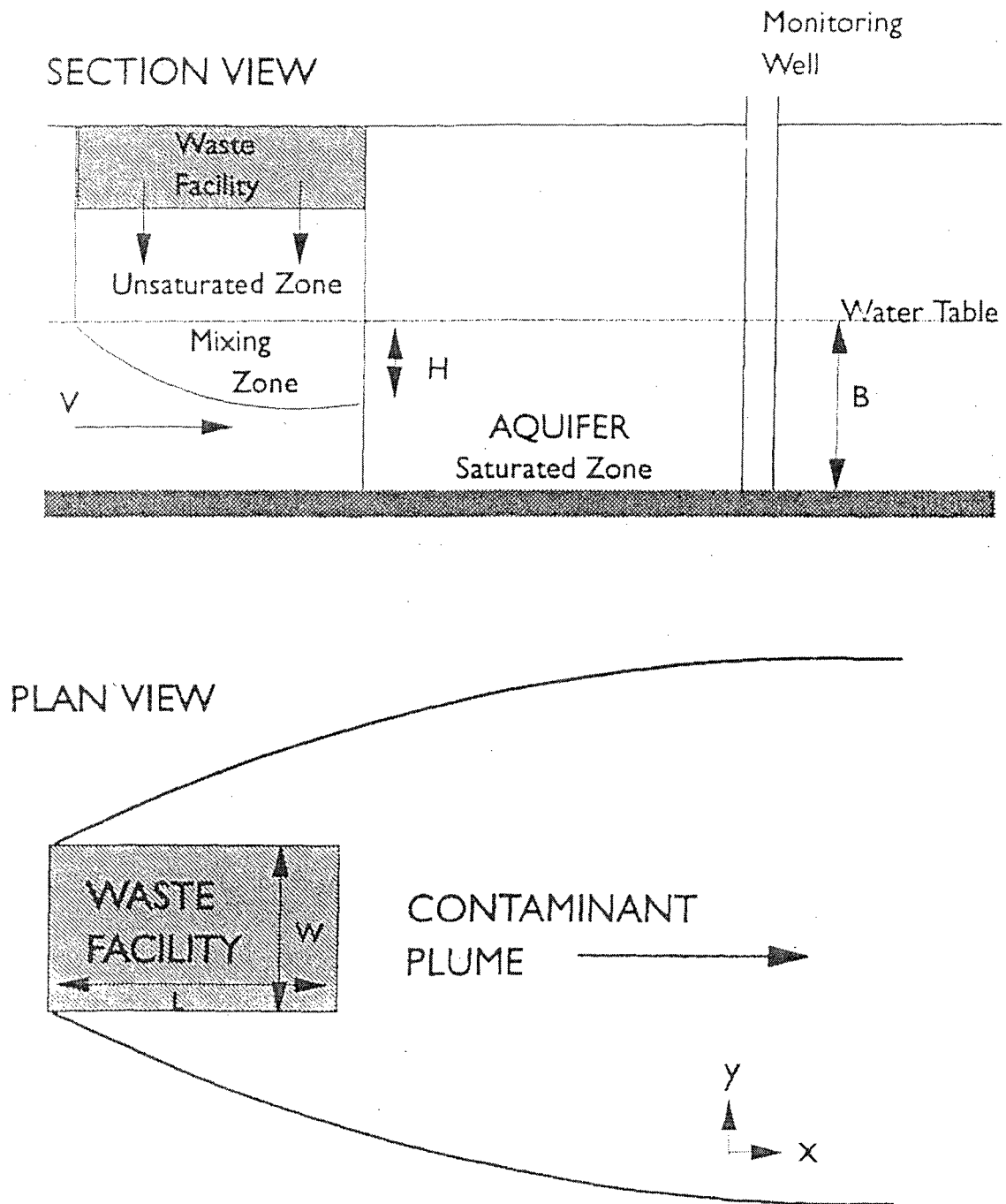
Figure 2.2 Waste facility schematic and MULTIMED geometry (after Salhouwa et al., 1990).
