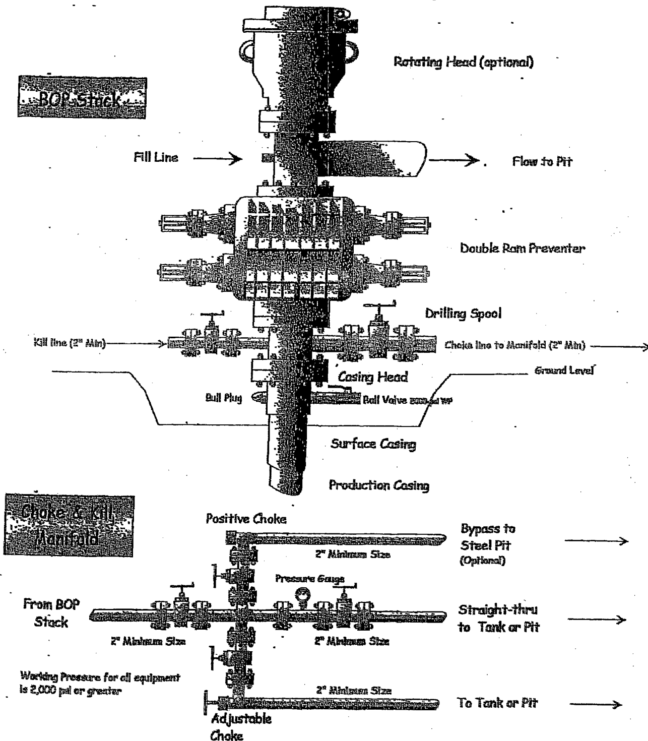
Exhibit #1 Typical BOP setup
