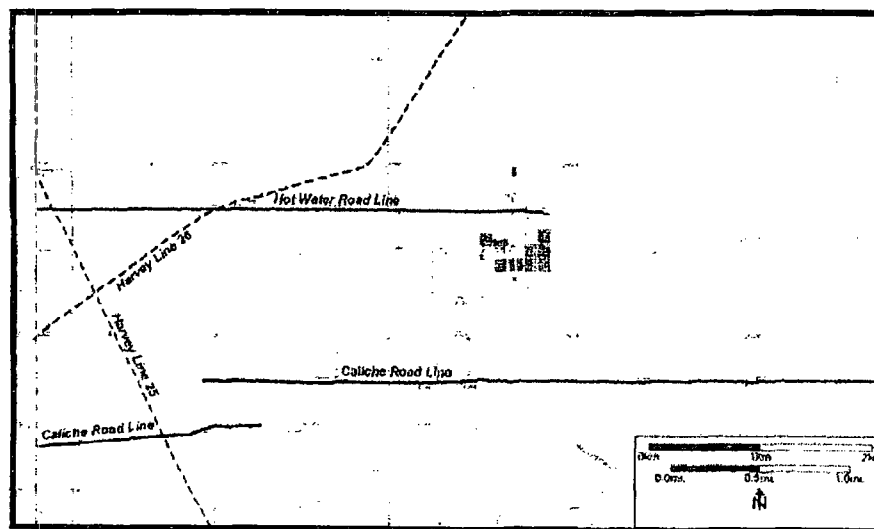
Figure 12. Seismic lines.
