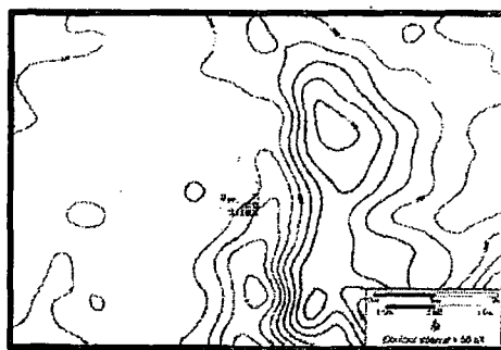
Figure 9. Residual magnetic contours (in nT) for the 200-m AGL survey.
