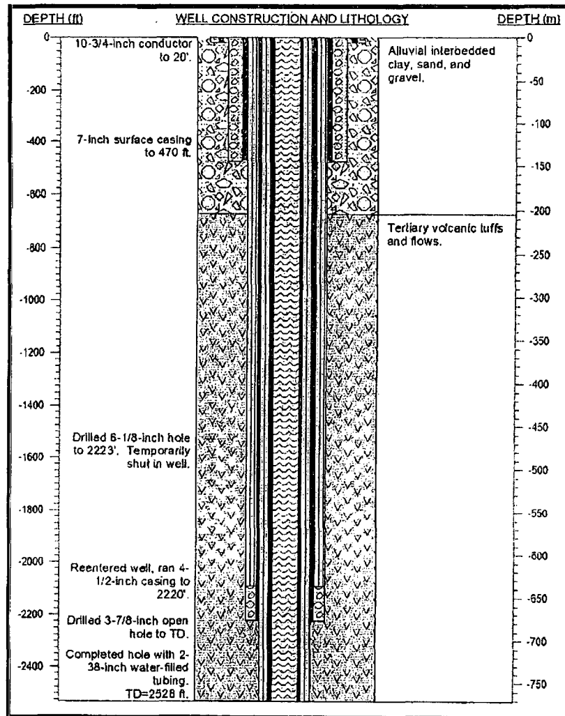
Figure 18. TG52-7 final completion schematic.
