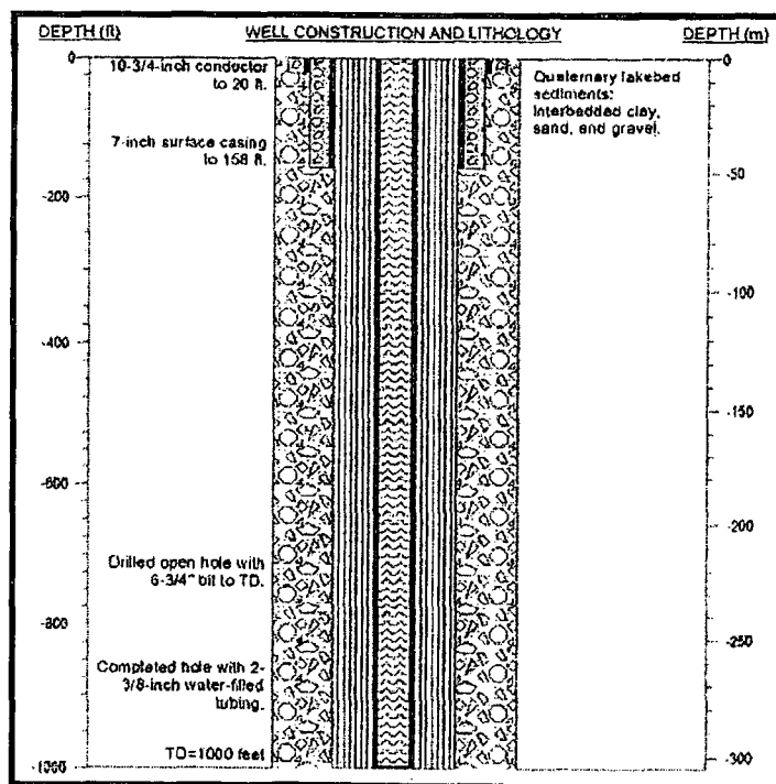
Figure 14. TG36-7 completion schematic.
