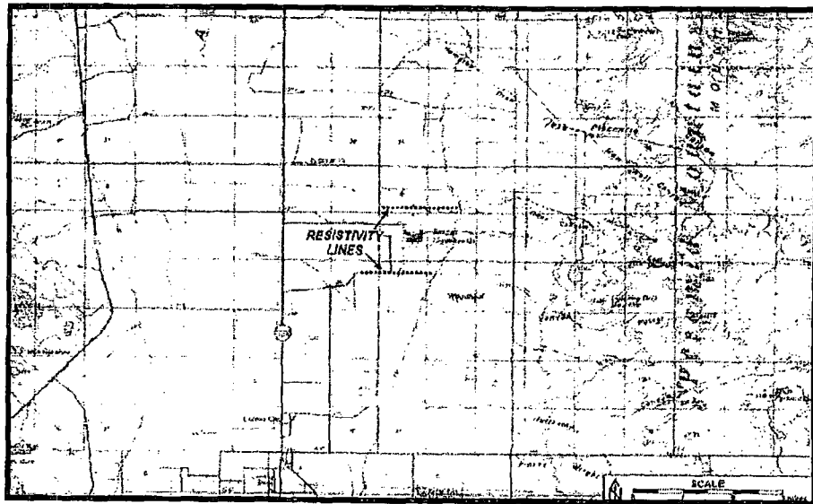
Figure 5. Location of dipole-dipole electrical resistivity lines.
