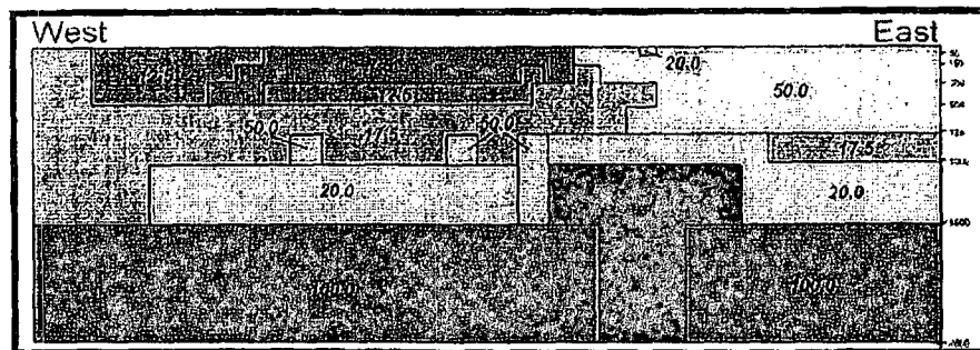
Figure 7. Resistivity block model for the Church Road line (from Mackelprang, 2001).
