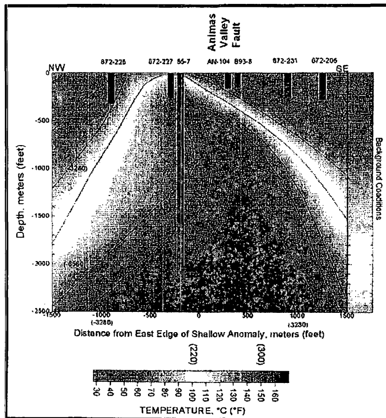
Figure 22. Initial conceptual model by Blackwell and Wisian (2001).
