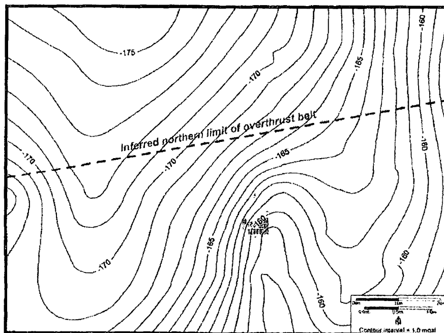
Figure 4. Simple Bouguer gravity contours.
