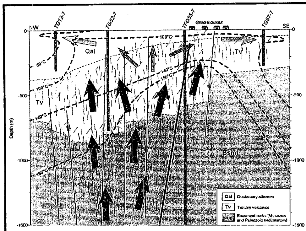
Figure 24. New conceptual model.
