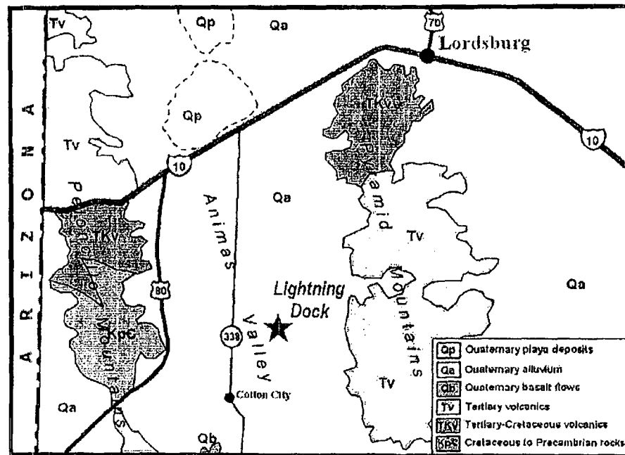
Figure 2. Geologic map of the Animas Valley region.
