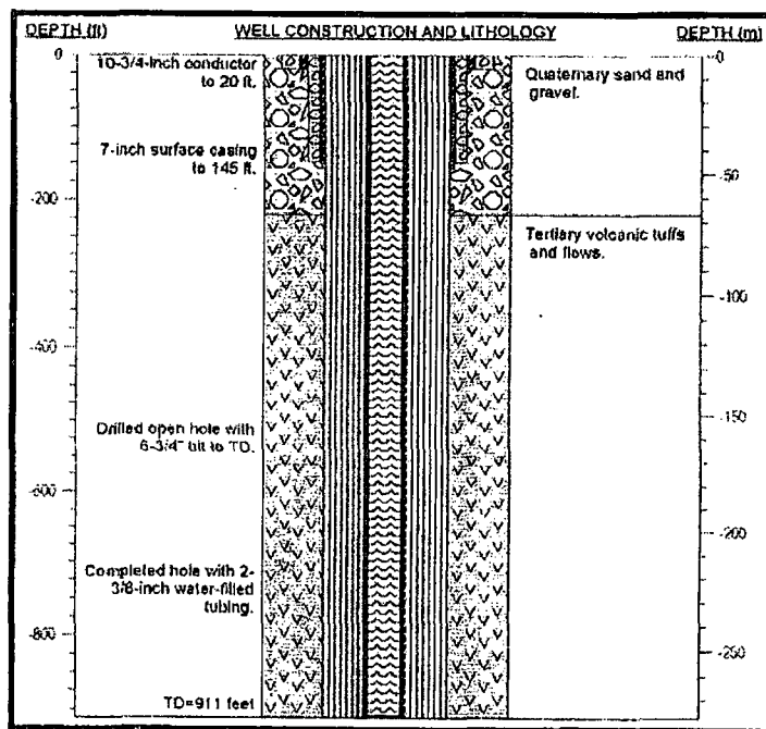
Figure 15. TG57-7 completion schematic.
