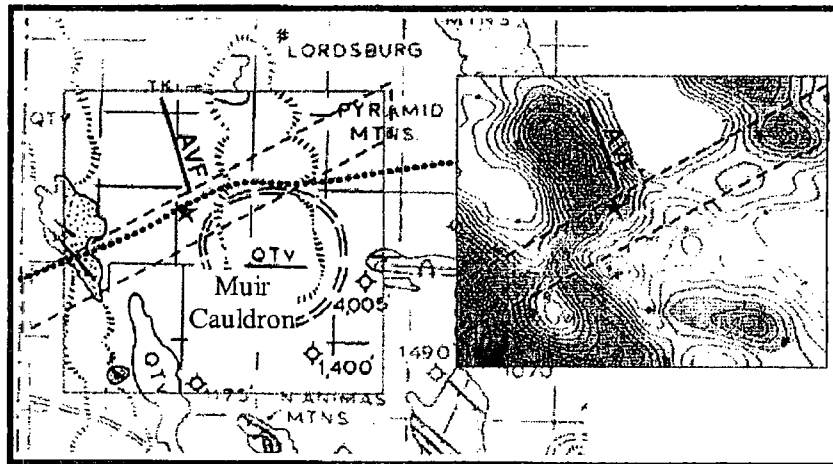
Figure 19. Integrated regional geology.
