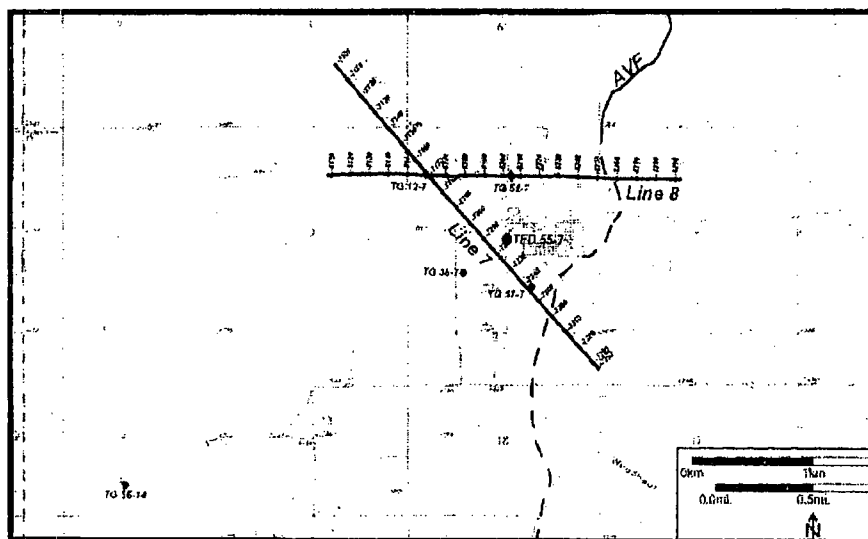
Figure 21. Seismic lines, 2004.
