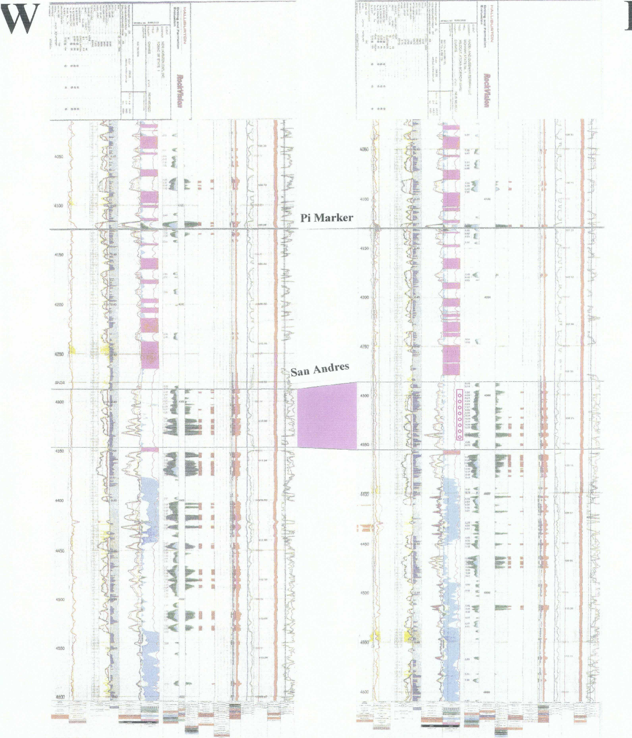
NADEL & GUSSMAN PERMIAN Hawkeye 29 State #1-H Stratigraphic San Andres X Section Chaves County, New Mexico SHG / MLH 2 / 15 / 2011
