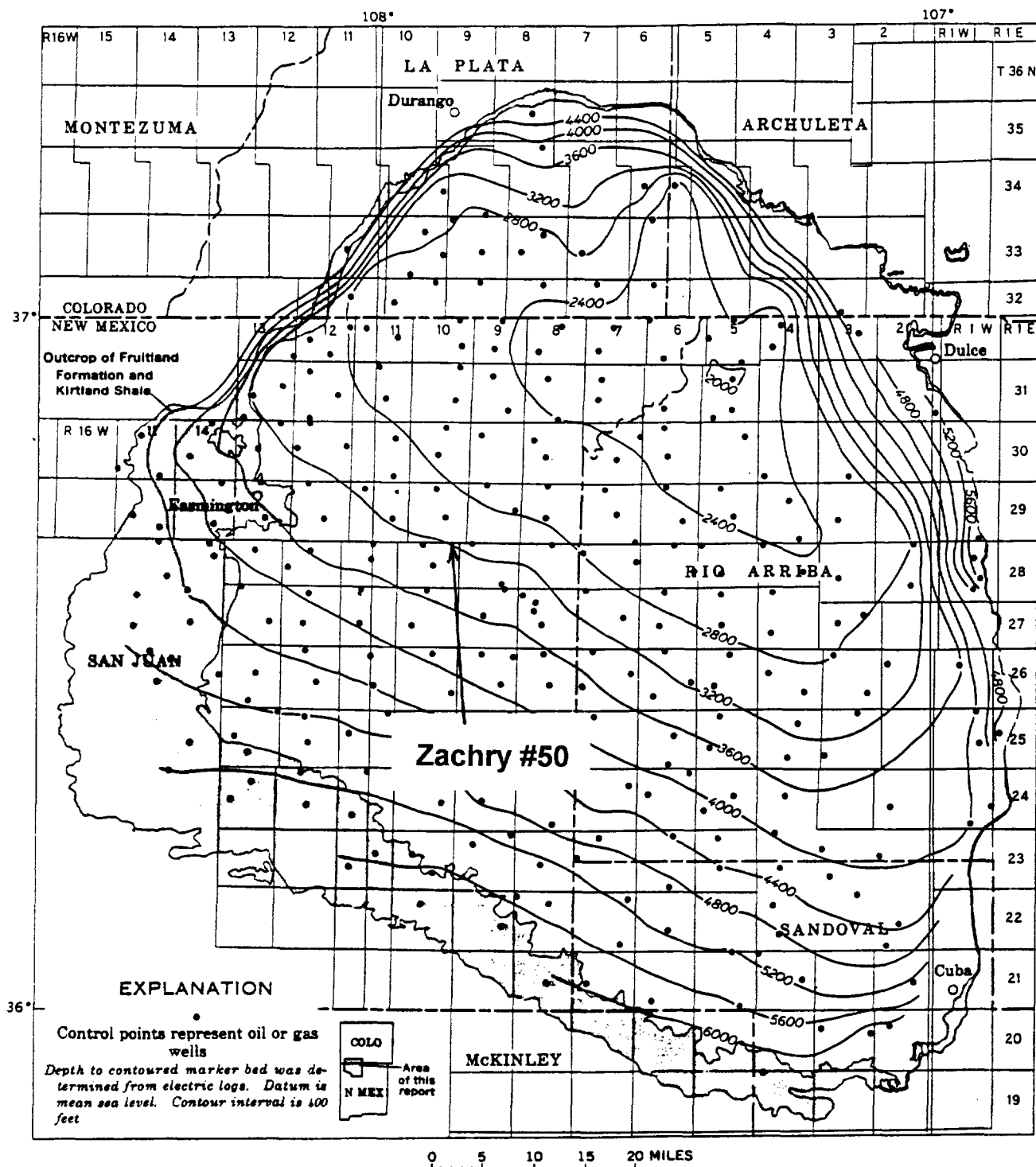
Contour map of the Huerfanito Bentonite Bed of the Lewis Shale.
