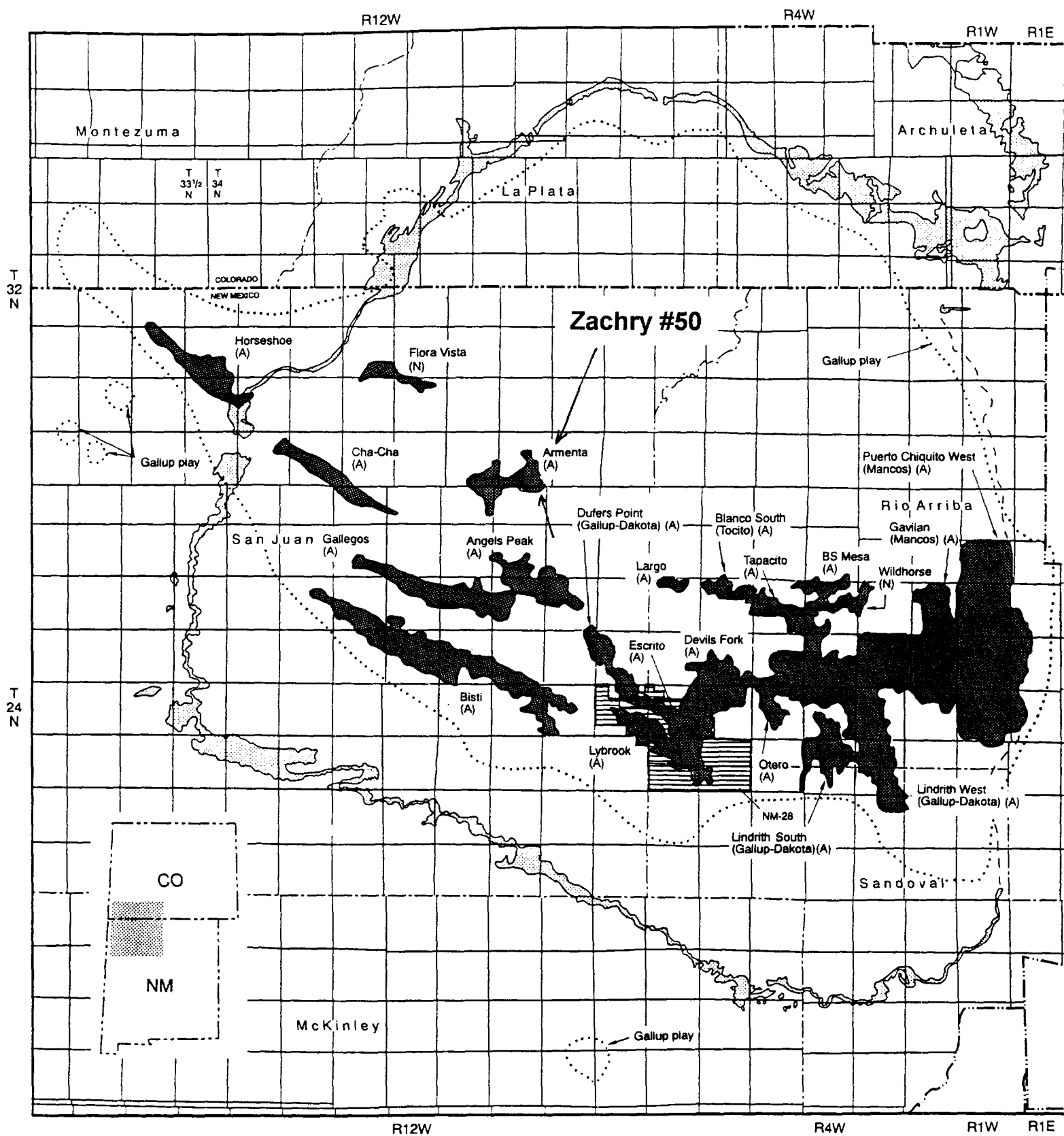
FIGURE SJ-4.1—Reservoirs and FERC-designated tight gas sand area for the Gallup producing interval reservoirs. Outcrop of the Pictured Cliffs Formation in New Mexico is from Dane and Bachman, 1965; outcrop of the Pictured Cliffs-Lewis Shale in Colorado is from Tweto, 1979.
