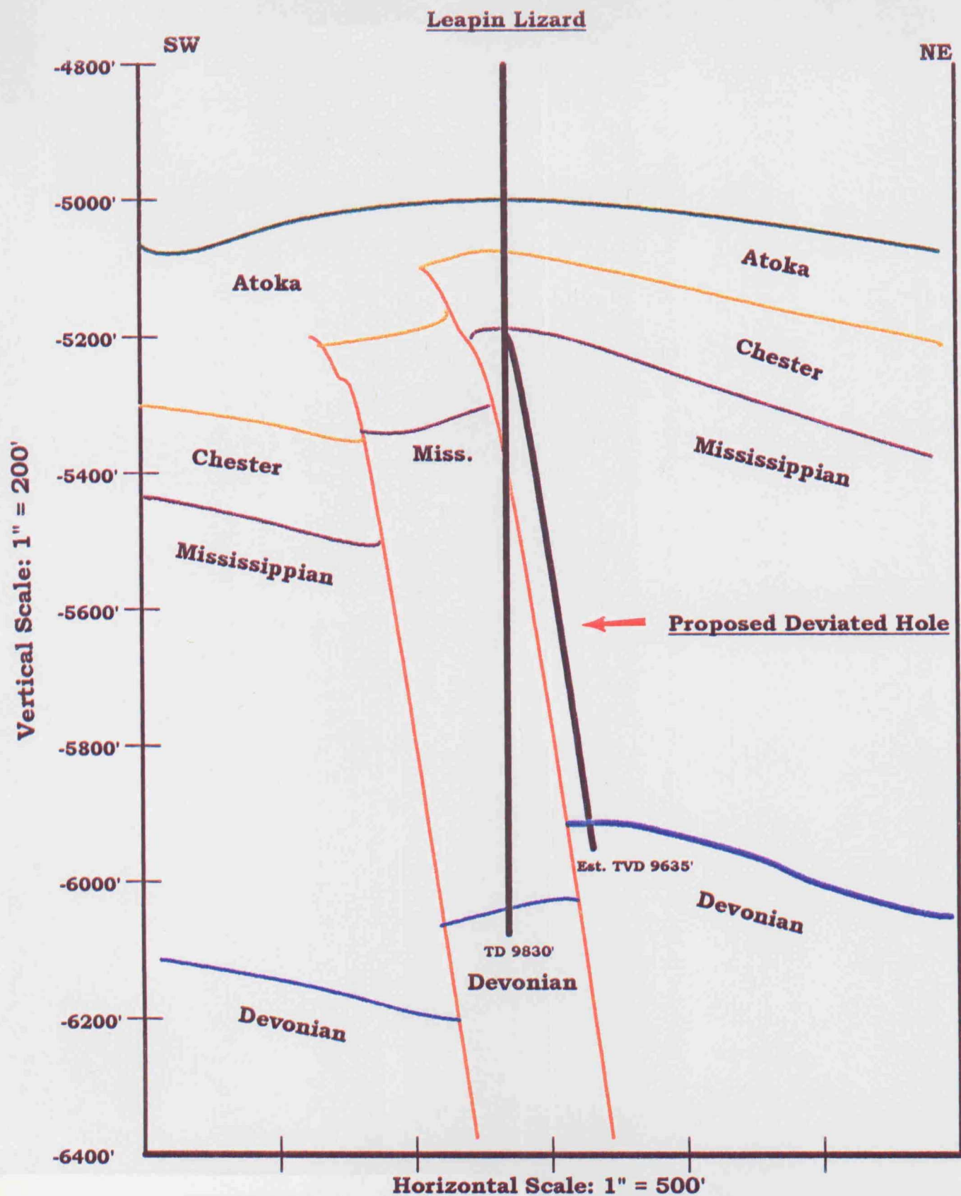
Marbob Energy Corporation Case 11306 - Exhibit C SW - NE Geologic Cross Section of Lower Paleozoics
