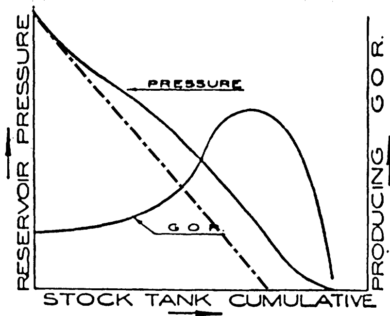
FIG. 161. Typical performance curves for an internal-gas-drive reservoir.
