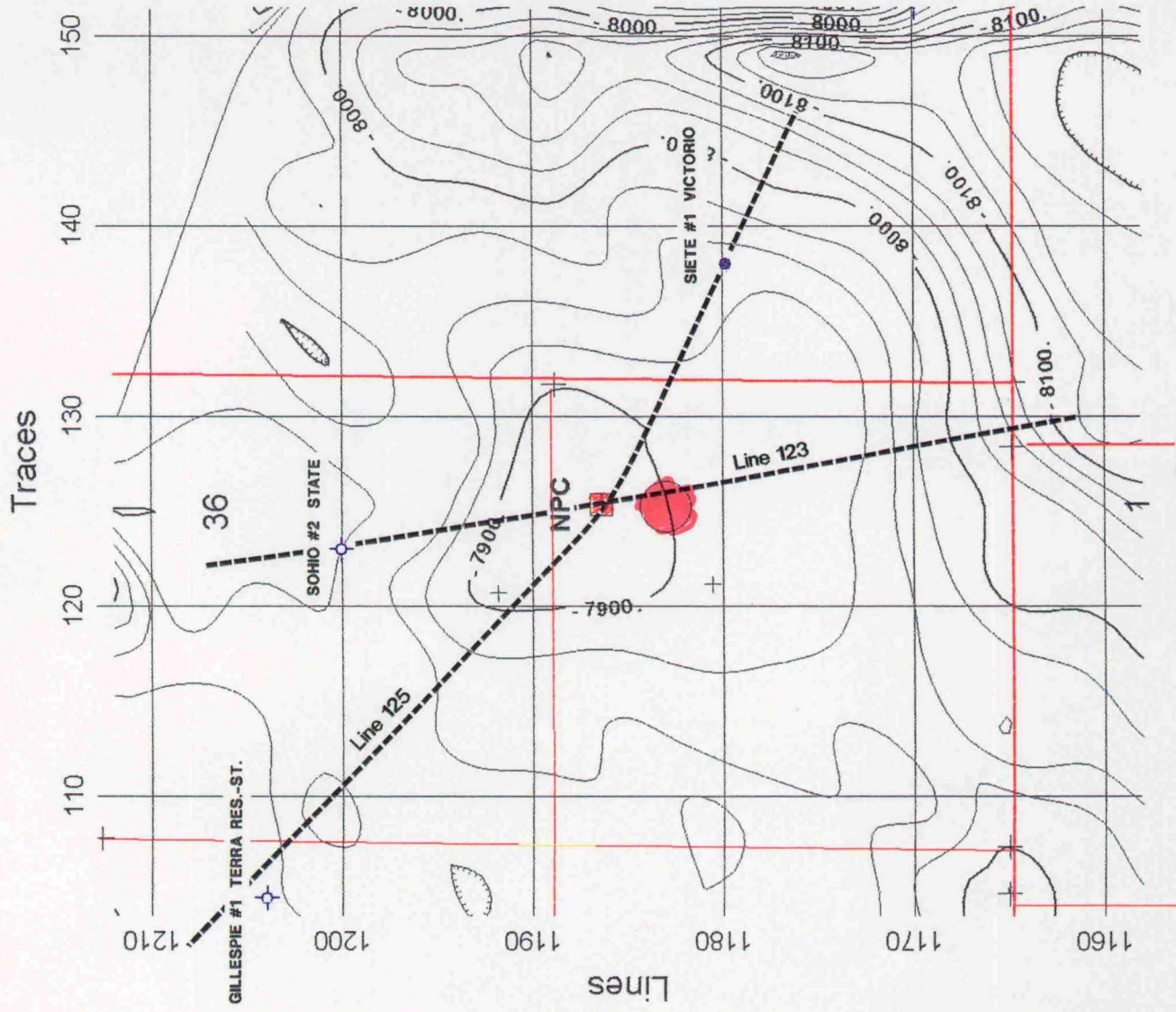
Ocho Prospect - Strawn Structure Map scale 1:1000 c.i. 25'
