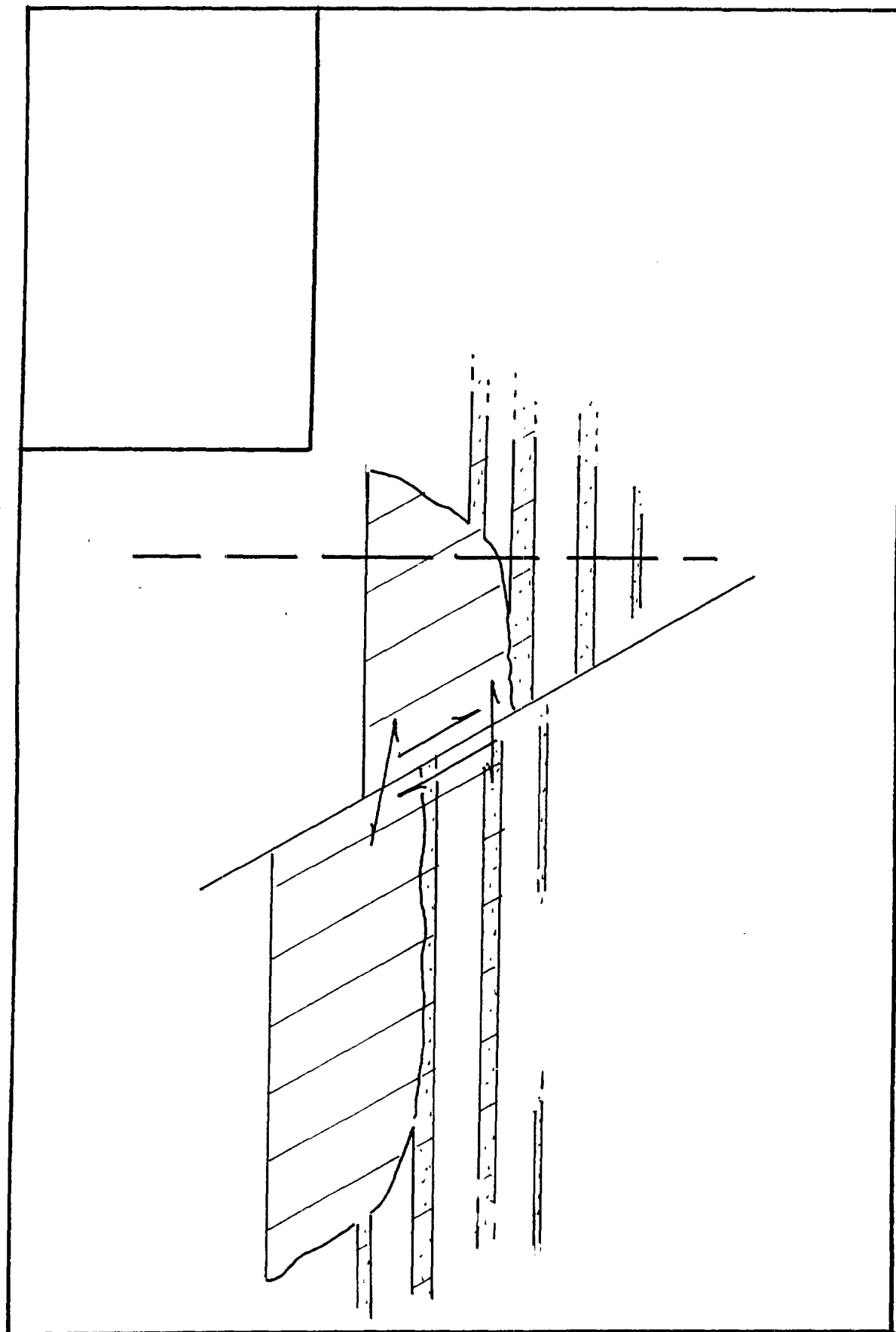
Schematic cross section no.1: Faulted distributary with cross fault communication
