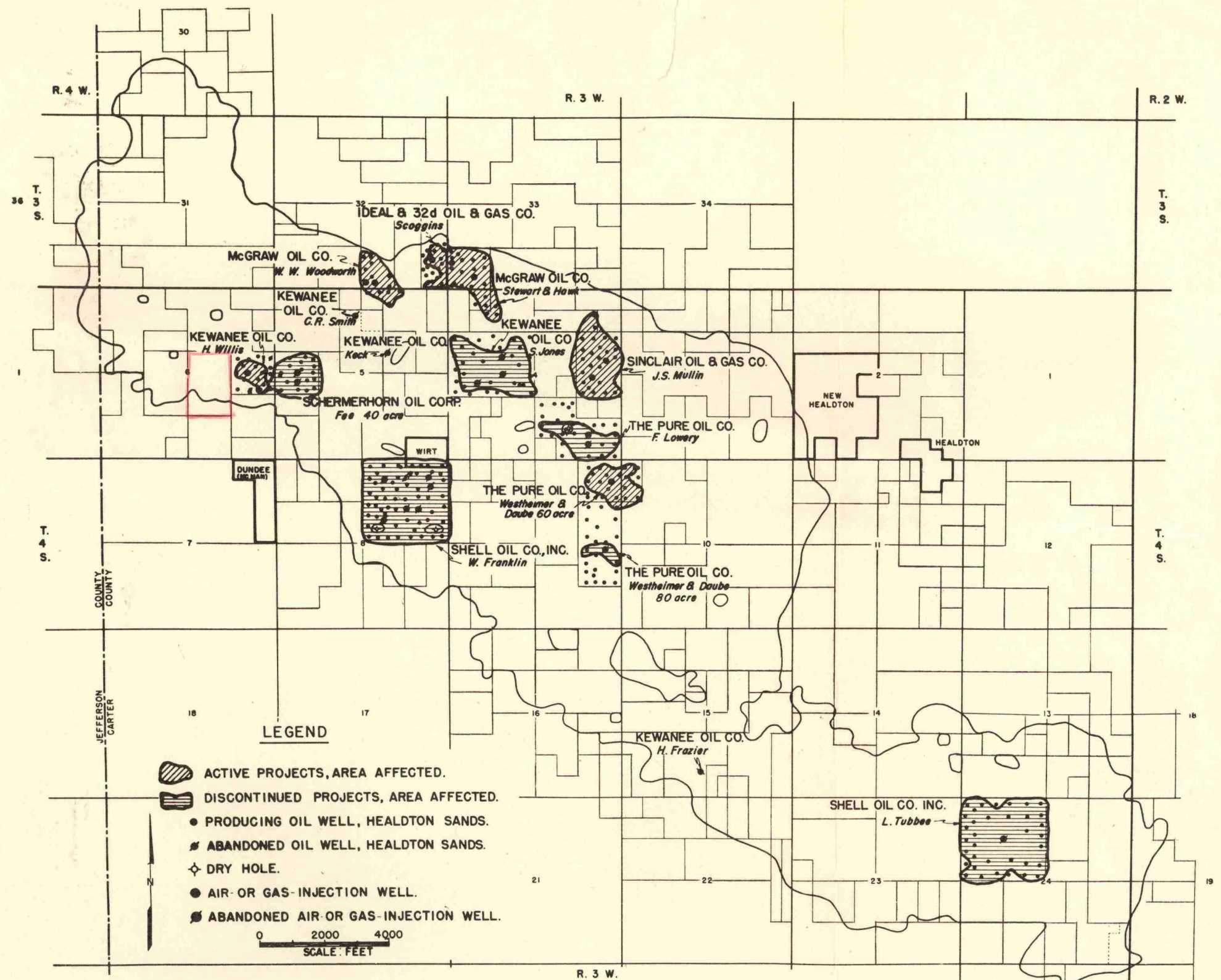
Figure 32. - Location of gas-injection projects and area affected, Healdton oil field, Carter County, Okla.
