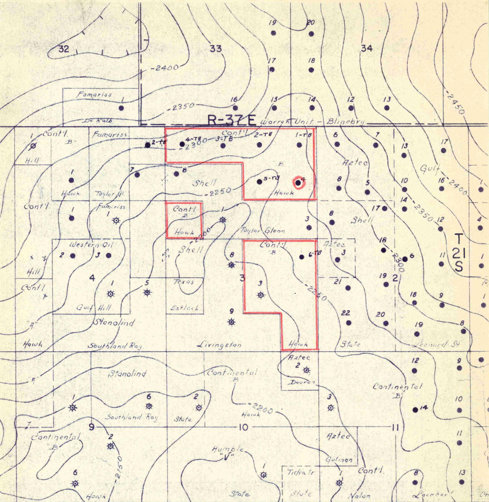
STRUCTURE PLAT T-21S, R-37E, LEA COUNTY, NEW MEXICO CONTOURED ON TOP OF BLINEBRY MARKER CONTOUR INTERVAL: 25' Scale: 1" = 2000'
