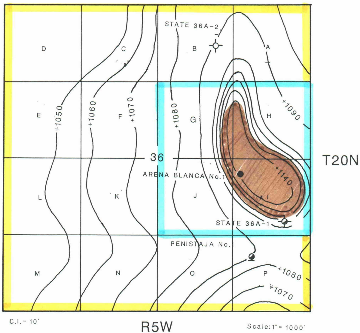
STRUCTURAL CONTOURS ON TOP OF ENTRADA SANDSTONE
