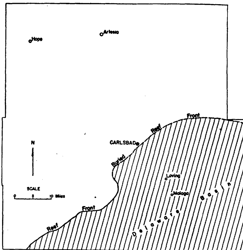
REEF FRONT AND EXTENT OF DELAWARE BASIN IN EDDY COUNTY, N. MEX. (After Walter B. Long, Am. Assoc. Petroleum Geologists Bull. , vol. 21, no. 7, 1937.)
