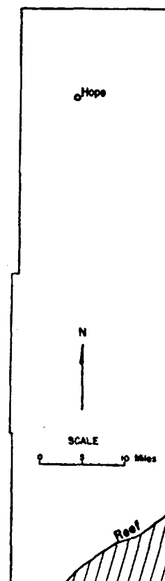
REEF FRONT IN EDDY COUNTY, N. MEX. (After Walcott, vol. 21, no. 7, 1937.)
