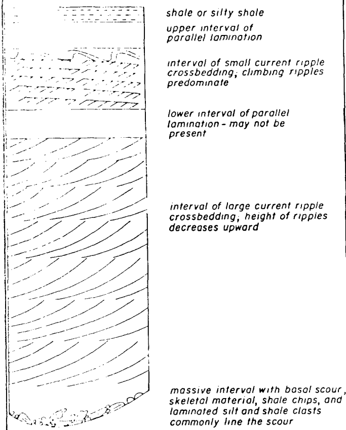
FIGURE 14. Major flow units characterize intermediate fan channel deposits in the Delaware Mountain Group. Major flow units range in thickness from 3–10 feet and most commonly have been partially truncated.
