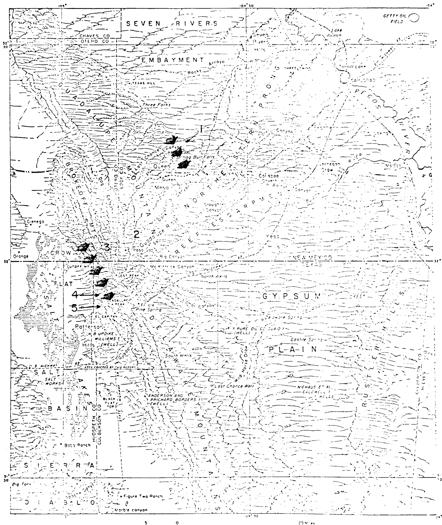
FIGURE 7. Physiographic map of Guadalupe Mountains and northwestern Delaware Basin. Compiled from various sources, including maps by U. S. Geological Survey and U. S. Forest Service. Arrows indicate approximate positions of ancient submarine canyon exposures. Locality (1) = Last Chance Sitting Bull Submarine Canyon; (2) = Shattuck Valley; (3) = West Dog Canyon; (4) = Shumard Canyon; (5) = Bone Canyon.
