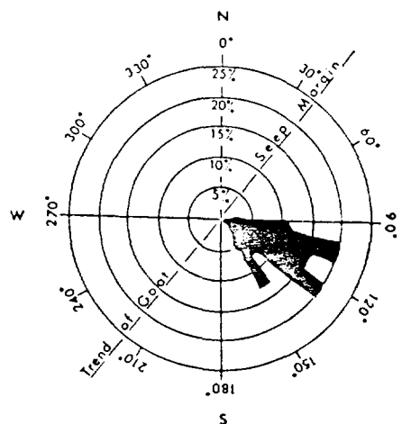
FIGURE 12. Rose diagram based on 616 measurements by Beck (1967).
