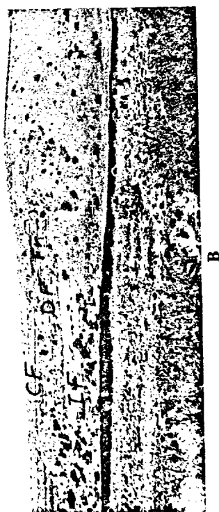
PLATE 16. Progradational-recessional fan-fringe cycles in Cherry Canyon and Bell Canyon Formations.
