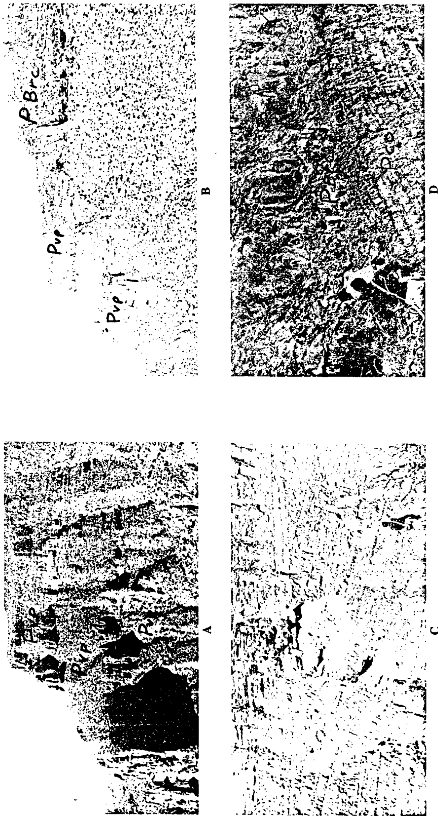
PLATE 3. Probable submarine canyon deposits in Shumard and Bone Canyons.
