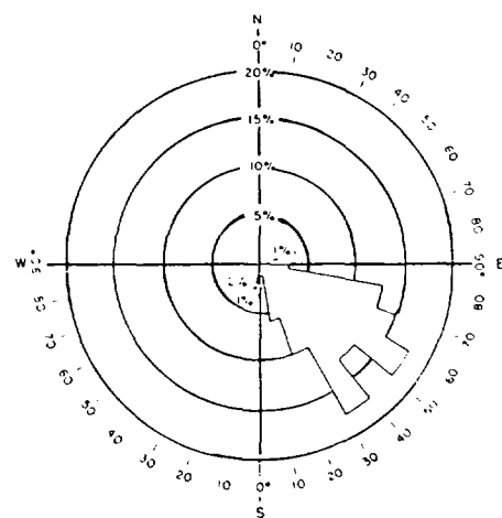
FIGURE 13. Based on 1595 measurements by Jacka.
