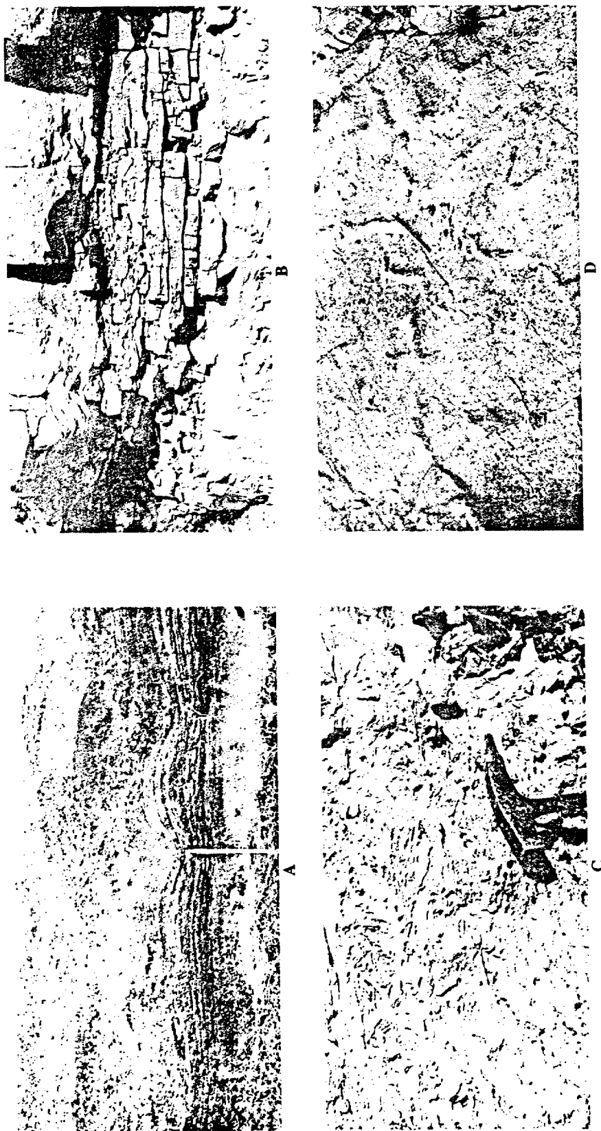
PLATE 22. Supratidal-algal flat deposits in Queen and Seven Rivers exposures.
