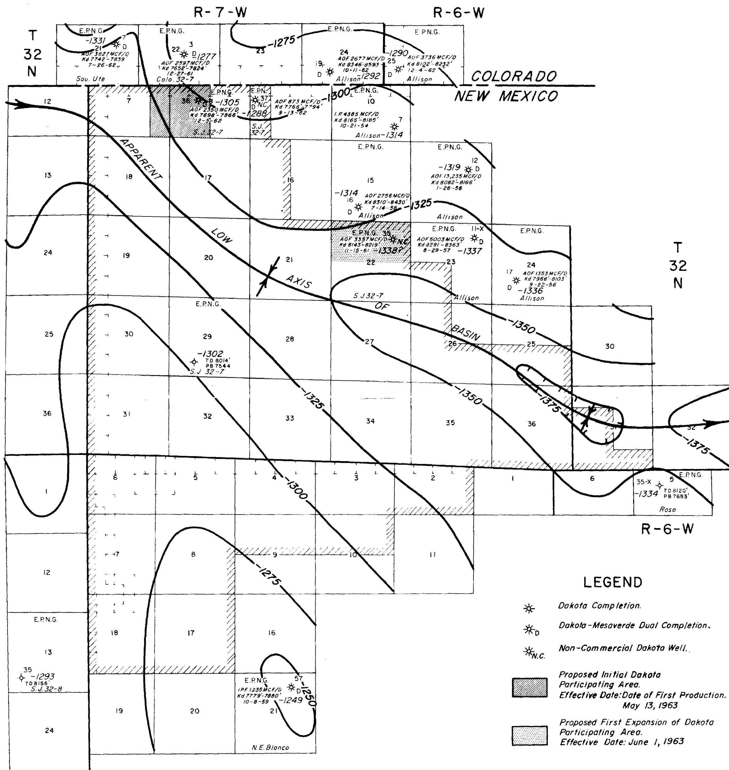
EXHIBIT "C" FIGURE NO. 1 SAN JUAN 32-7 UNIT SAN JUAN COUNTY, NEW MEXICO DAKOTA STRUCTURE MAP HORIZON: TOP OF GRANEROS SHALE DATUM: DERRICK FLOOR ELEVATION CONTOUR INTERVAL = 25 FEET
