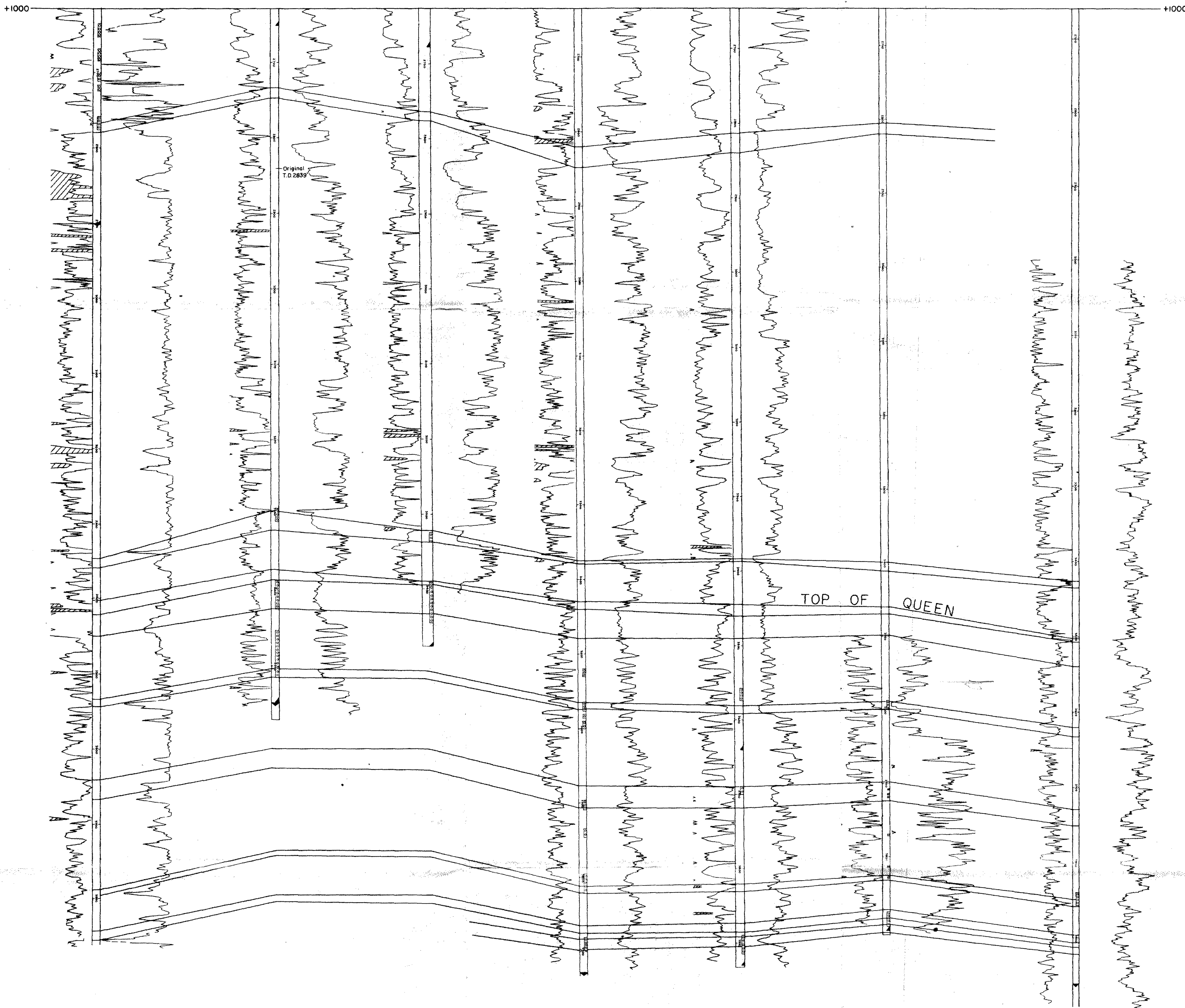
WEST-EAST CROSS-SECTION PART OF SHUGART POOL EDDY COUNTY, NEW MEXICO NO HORIZONTAL SCALE THE ATLANTIC REFINING COMPANY
