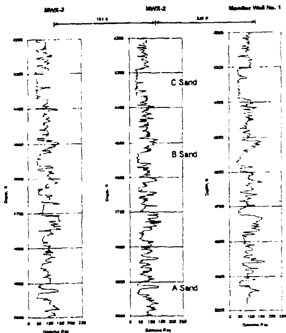
Figure 2: Cross-Section of M-Site Target Sand Intervals
