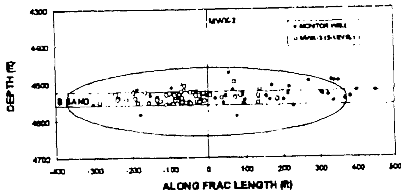
Figure 8c: Profile Map 45 Minutes After Initiating Injection (18-Minute Injection Plus 27-Minute Shut-In)
