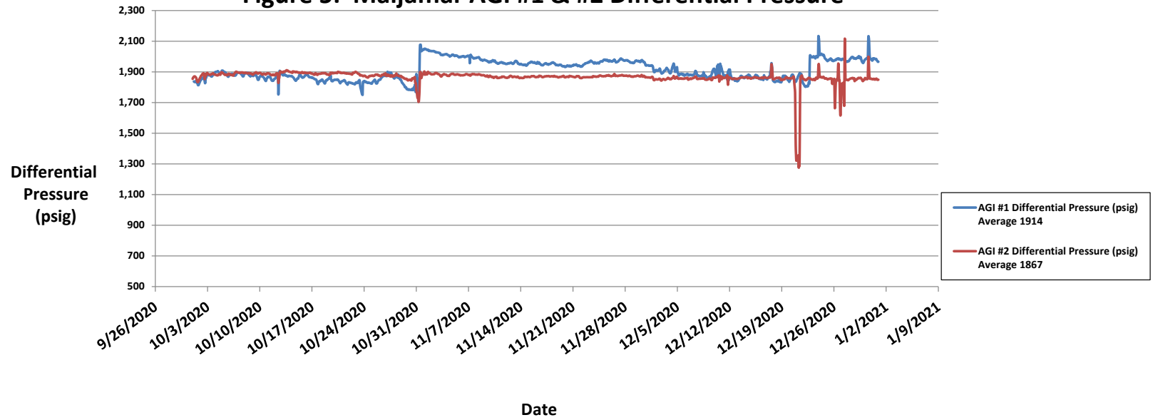
Figure 5: Maljamar AGI #1 & #2 Differential Pressure
