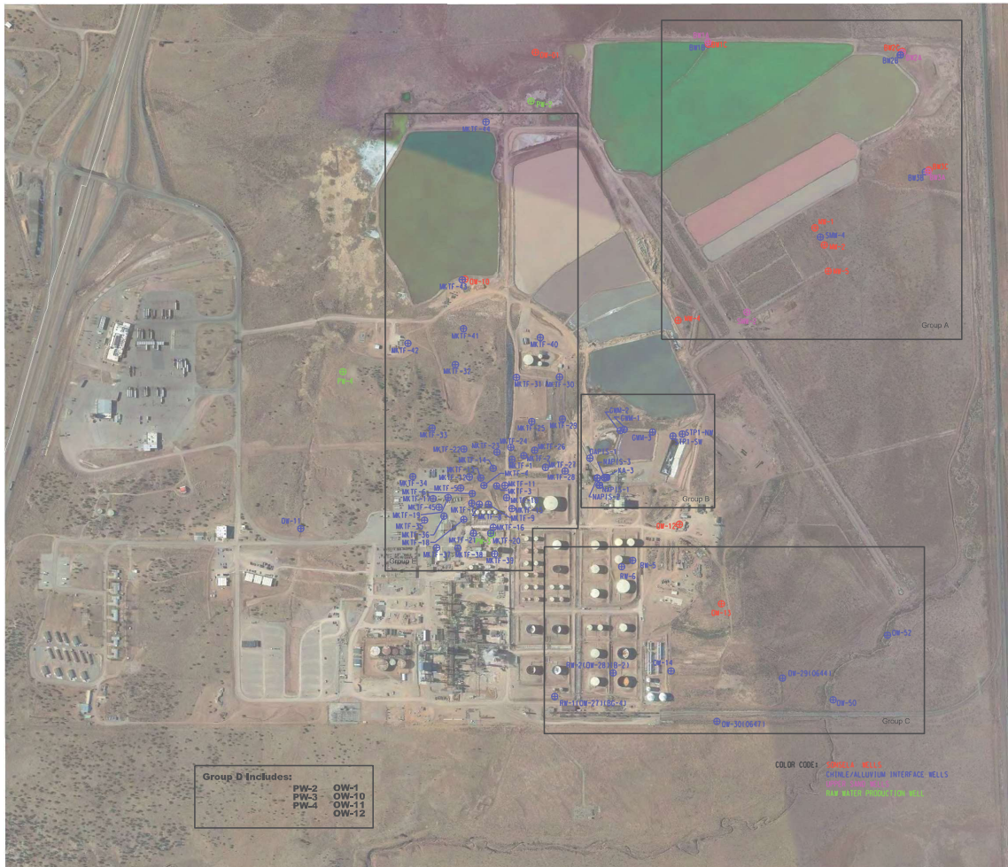
Figure 6 FACILITIES AND WELL GROUPS - 2016 WESTERN REFINING - GALLUP REFINERY
