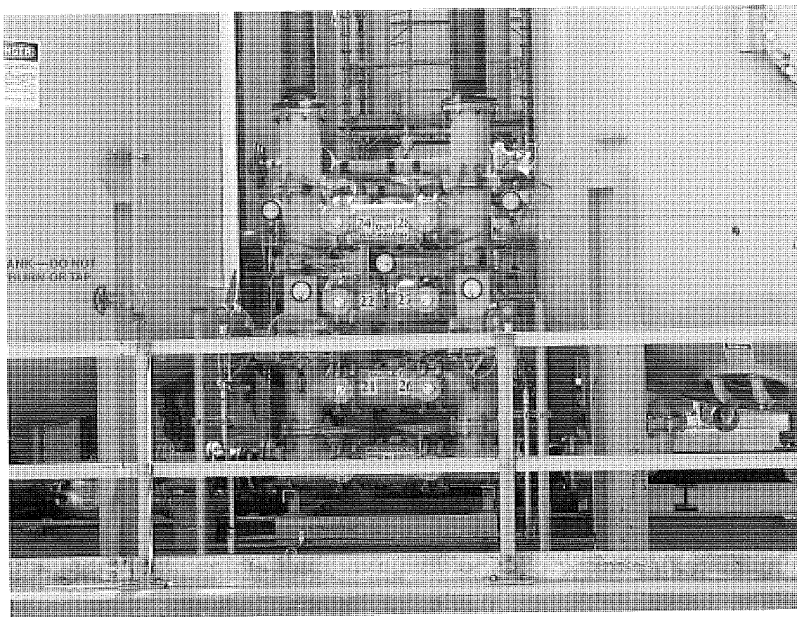
Photo 4: Updated carbon treatment system piping manifold – closeup.
