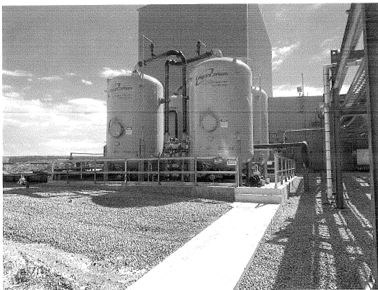
Photo 2: Upgraded four 20,000-pound carbon treatment system.
