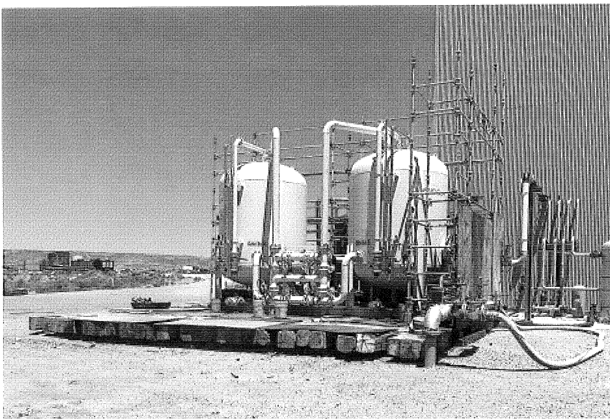
Photo 1: Original two 10,000-pound wastewater treatment system carbon system.
