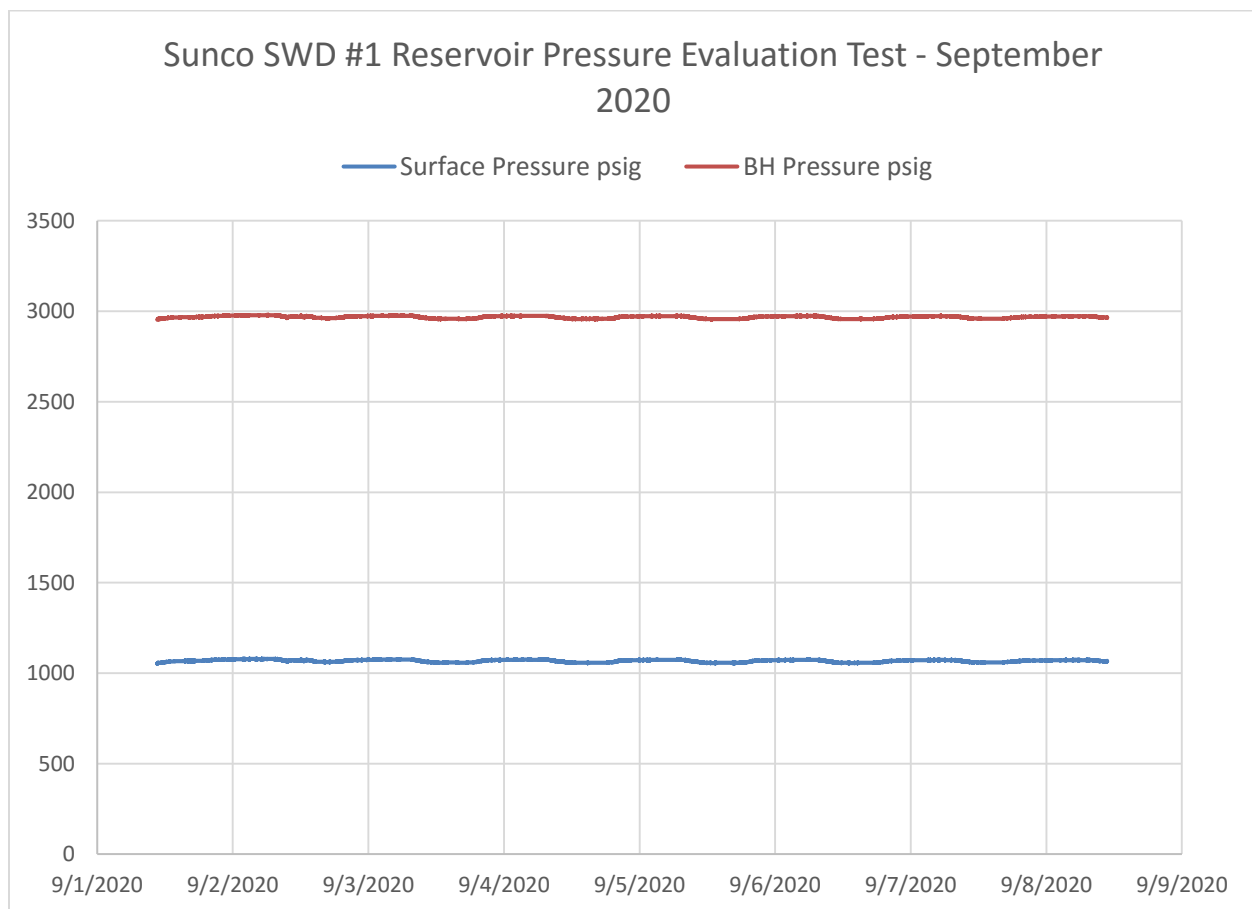
Figure 2 Calculated BH Pressure vs. Time
