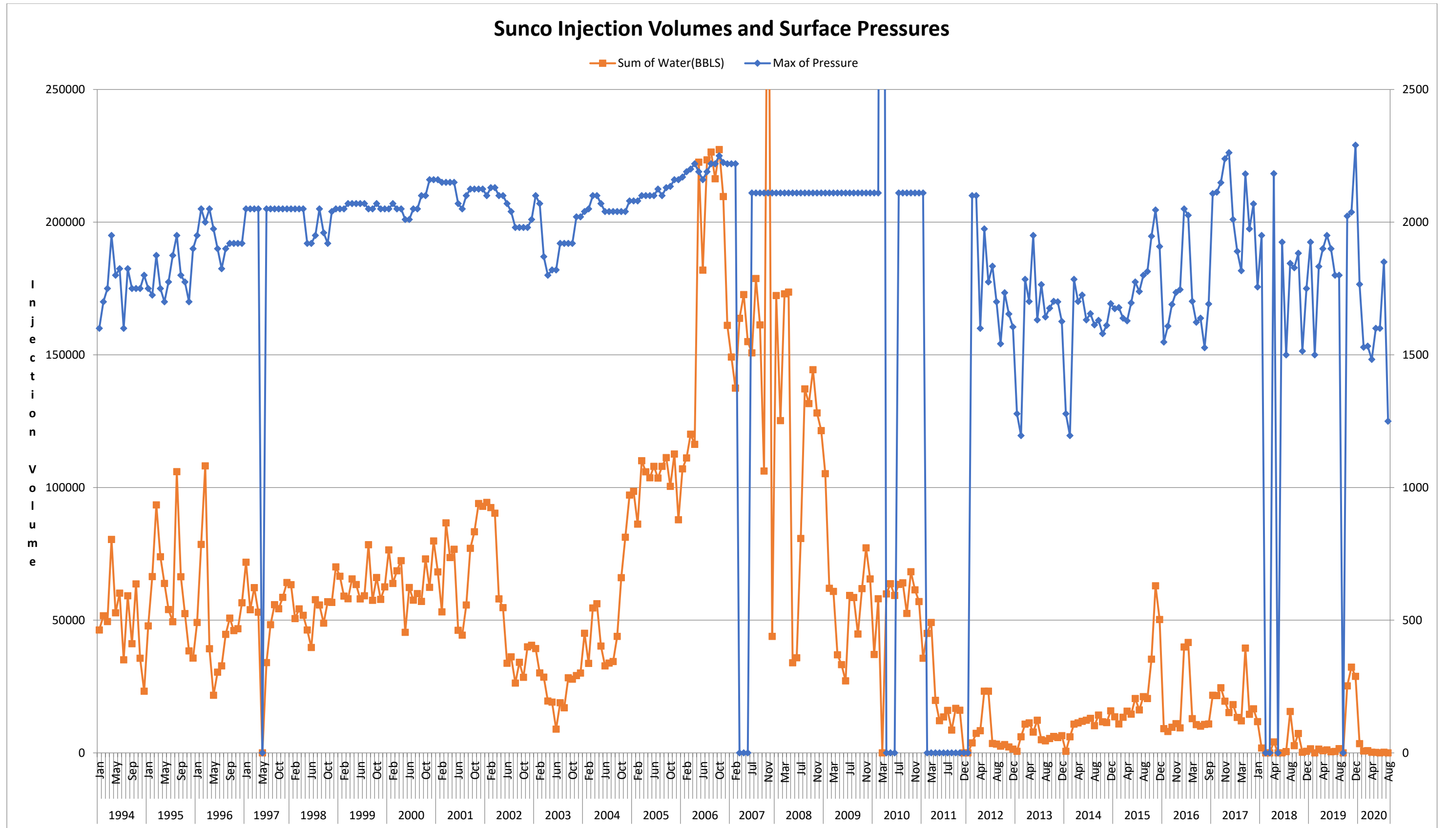
Figure 2 Injection and Pressure Plot
